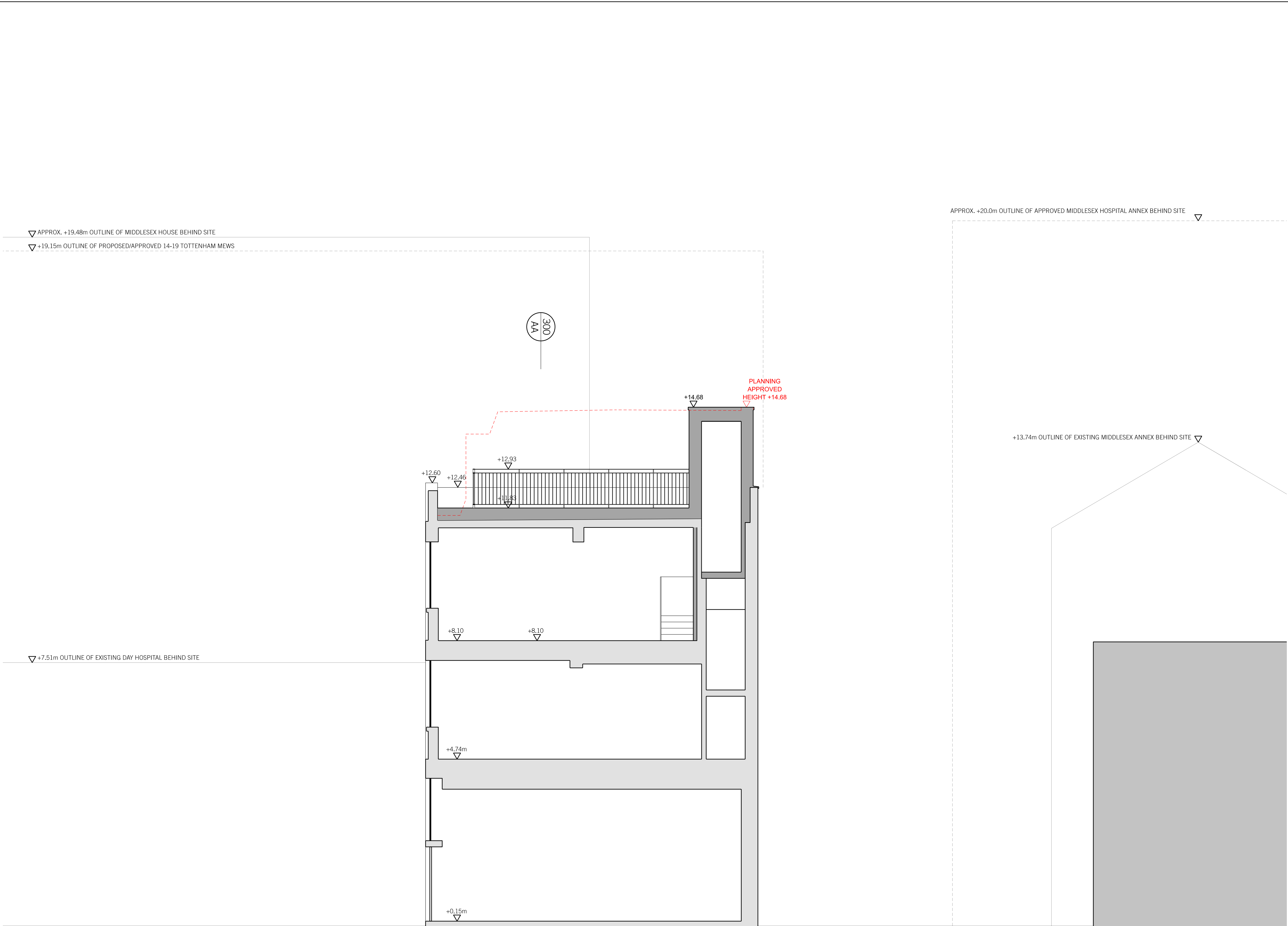
01: PROPOSED SECTION BB SCALE 1:50
