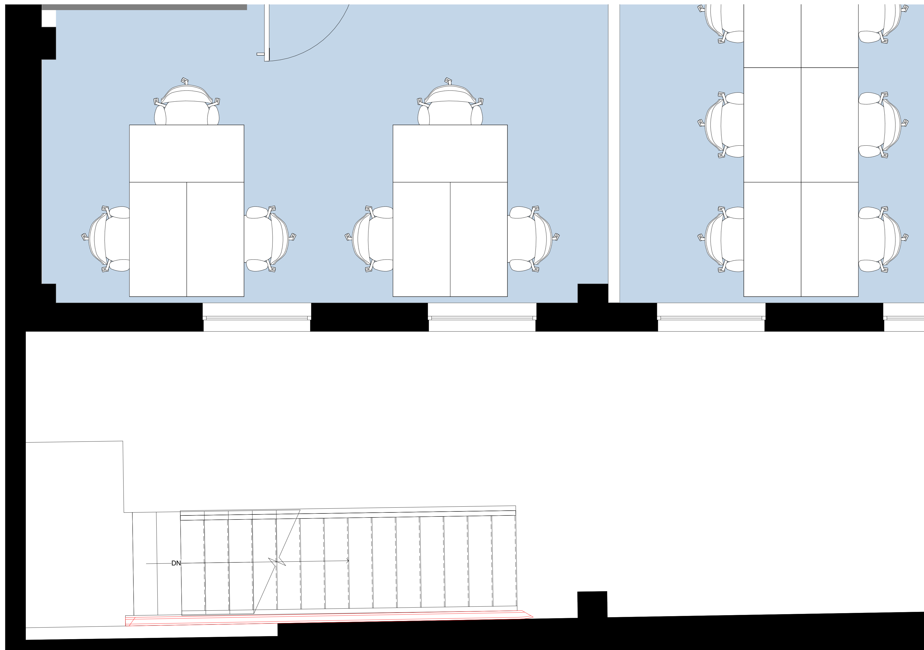
3 General Arrangement - Ground Floor Bike Store 1 : 20
