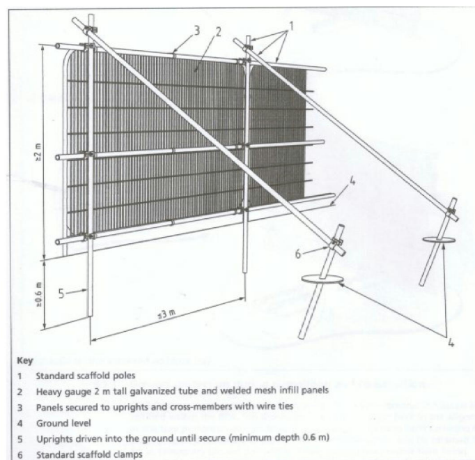
Fig. 1 Protective fencing in accordance with B.S. 5837
