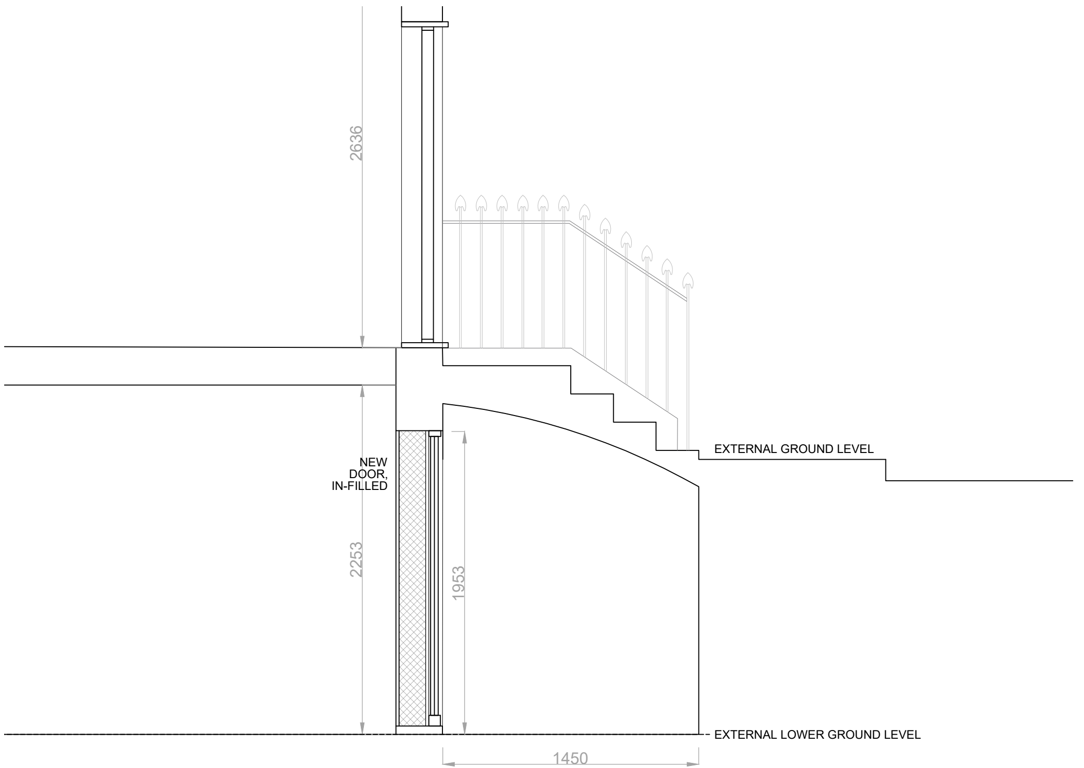
Lightwell End Elevation - 1:25
