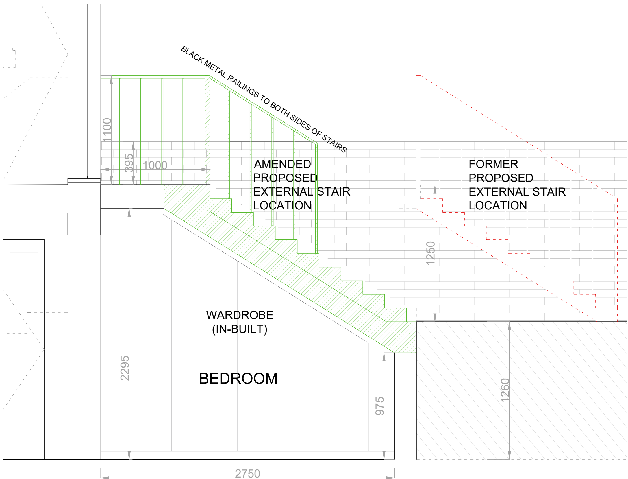
Proposed Section 02 - 1:50
