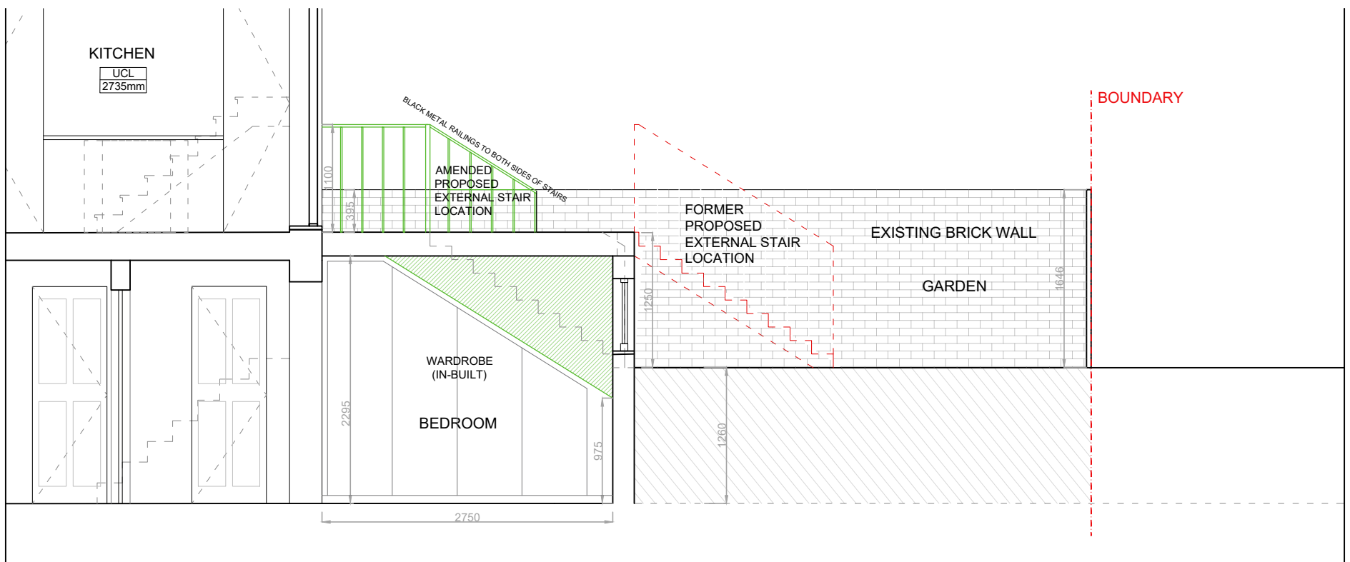
Proposed Section 01 - 1:50
