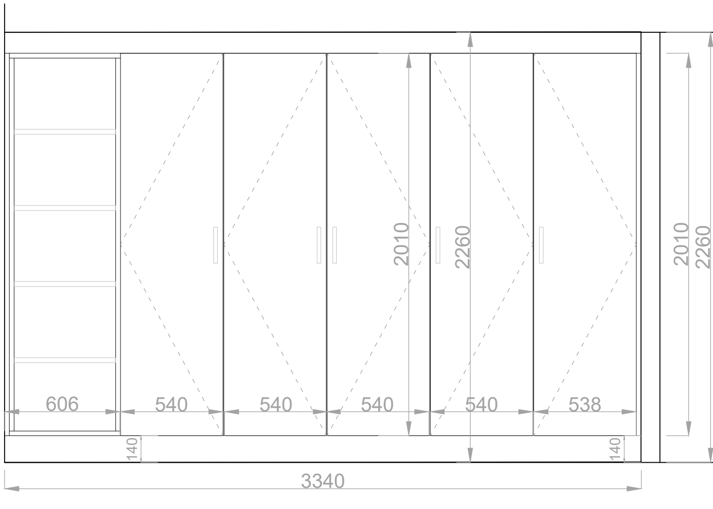
Lower Ground Bedroom 2 - Wardrobe Elevation - 1:20
