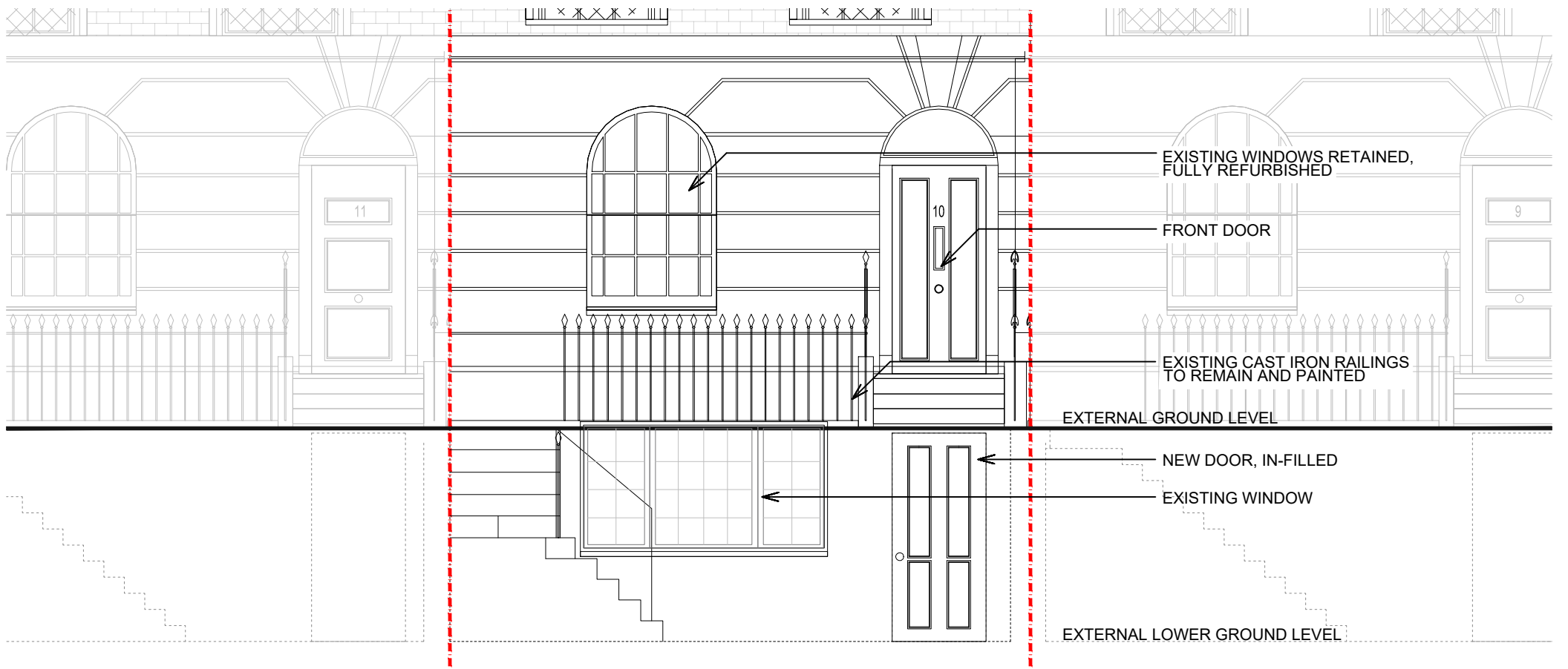
Front Elevation (North East) 1:50
