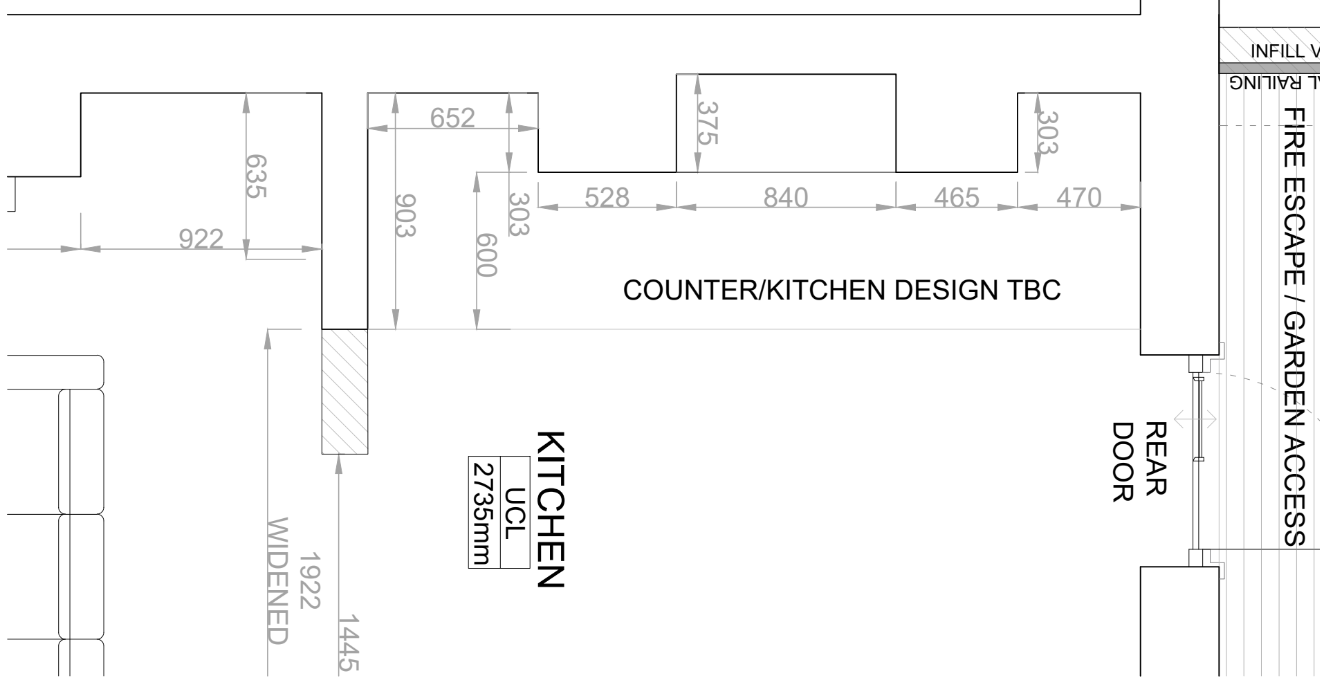
Kitchen Reference plan - 1:20
