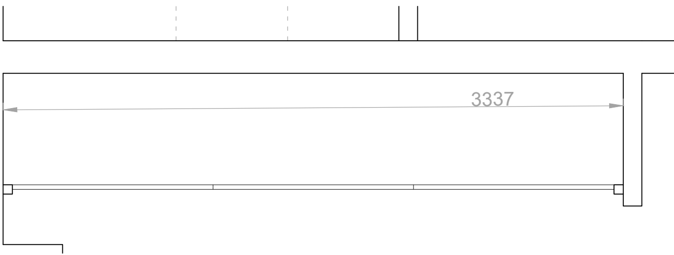
Lower Ground Bedroom 2 - Wardrobe Plan - 1:20
