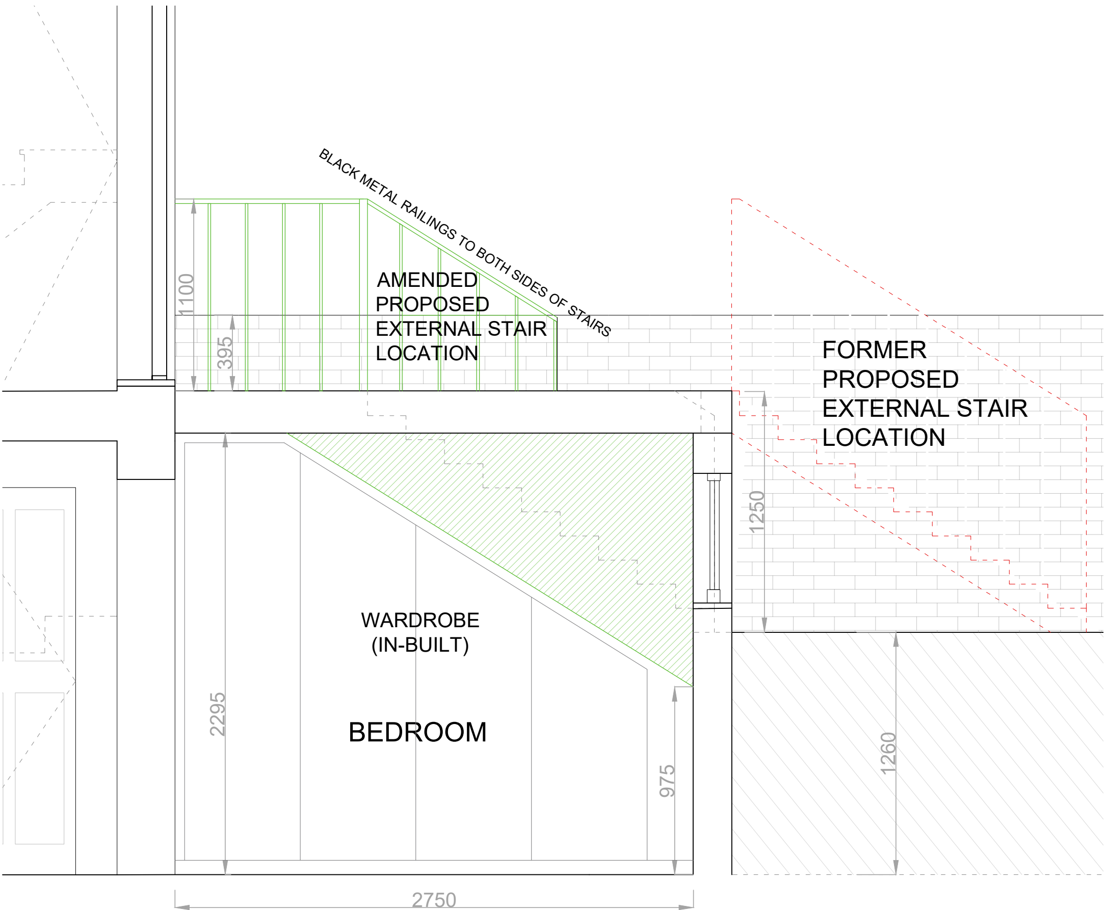
Proposed Section 01 - 1:50
