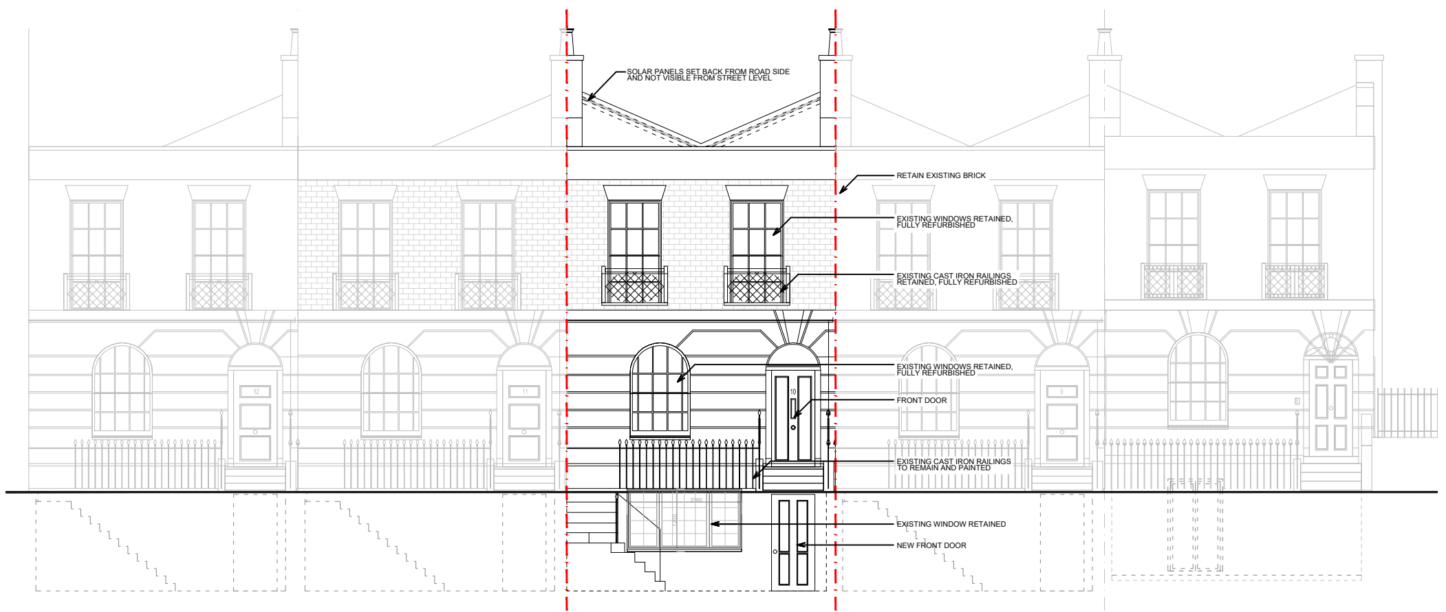
Front Elevation (South West) 1:100
