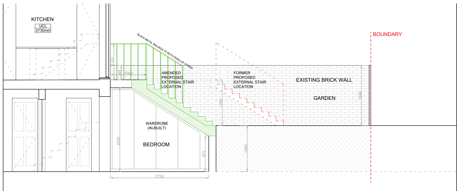
Proposed Section 02 - 1:50
