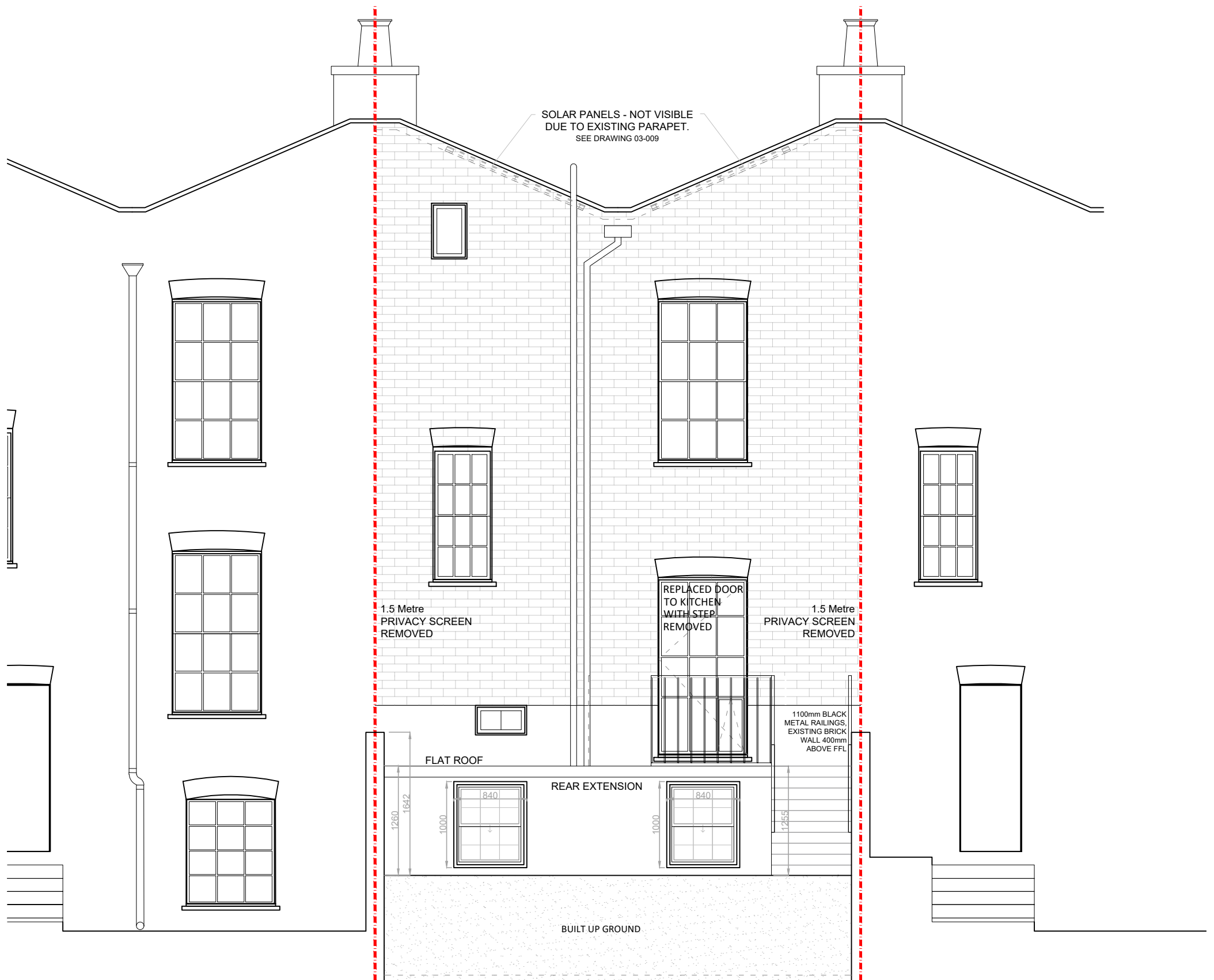
Rear Elevation (South West) 1:100
