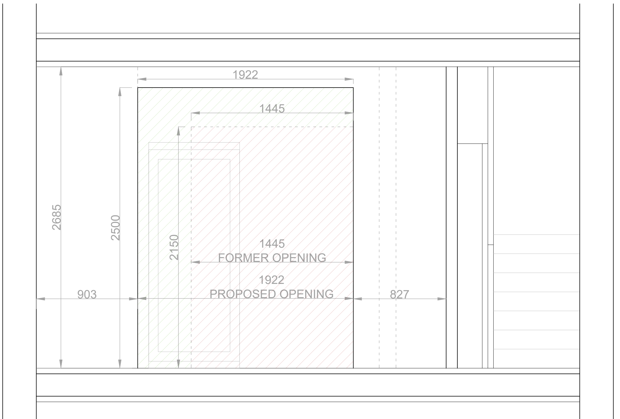
Proposed Opening Elevation - 1:20
