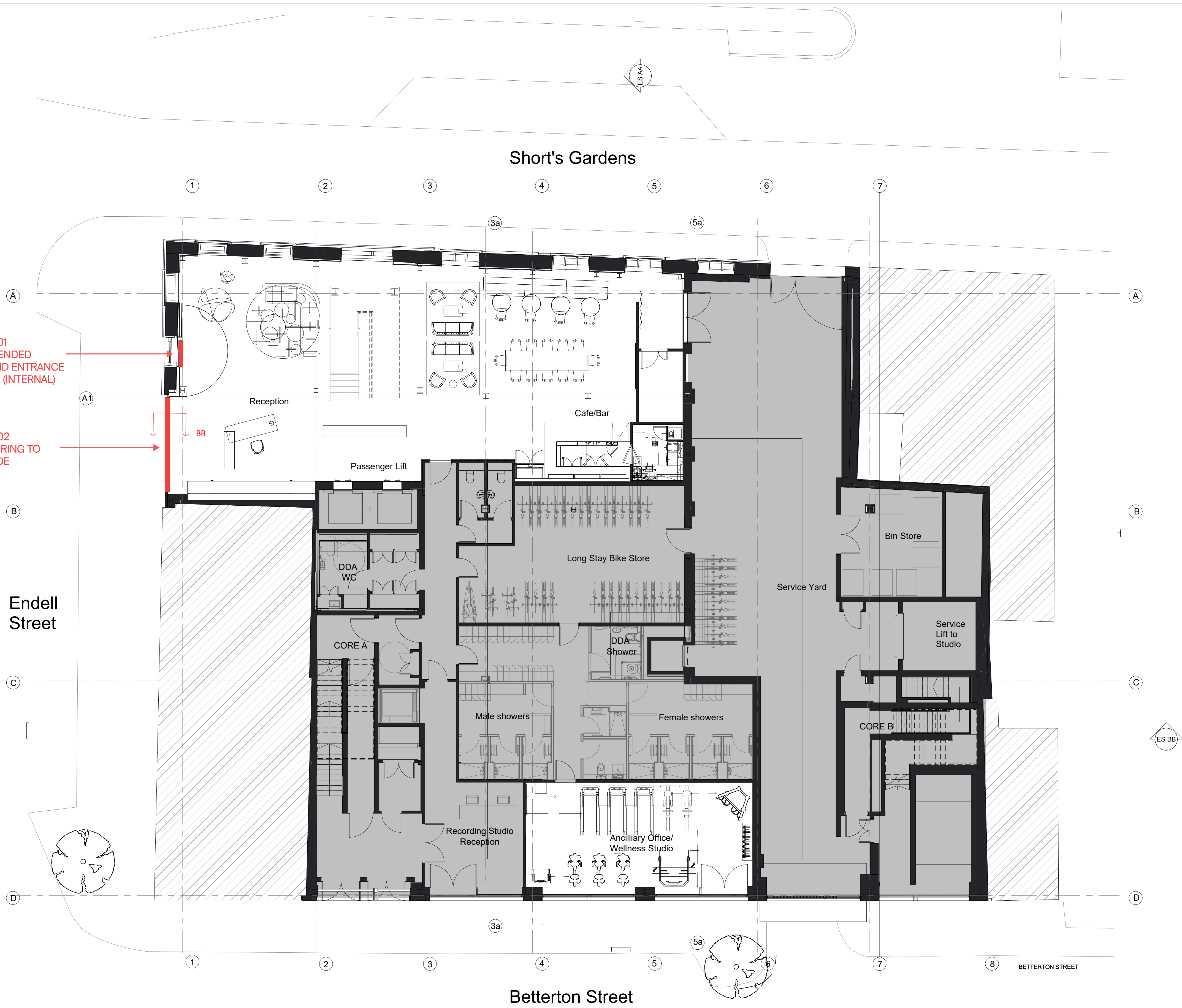
Ground Floor Plan -Proposed Scale: 1:100
