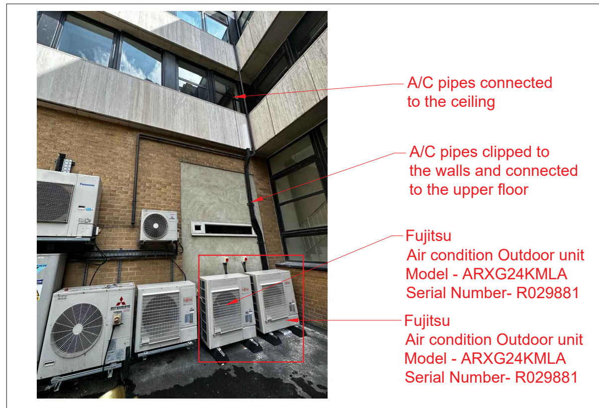
EXISTING OUTDOOR A/C UNITS to be retained
