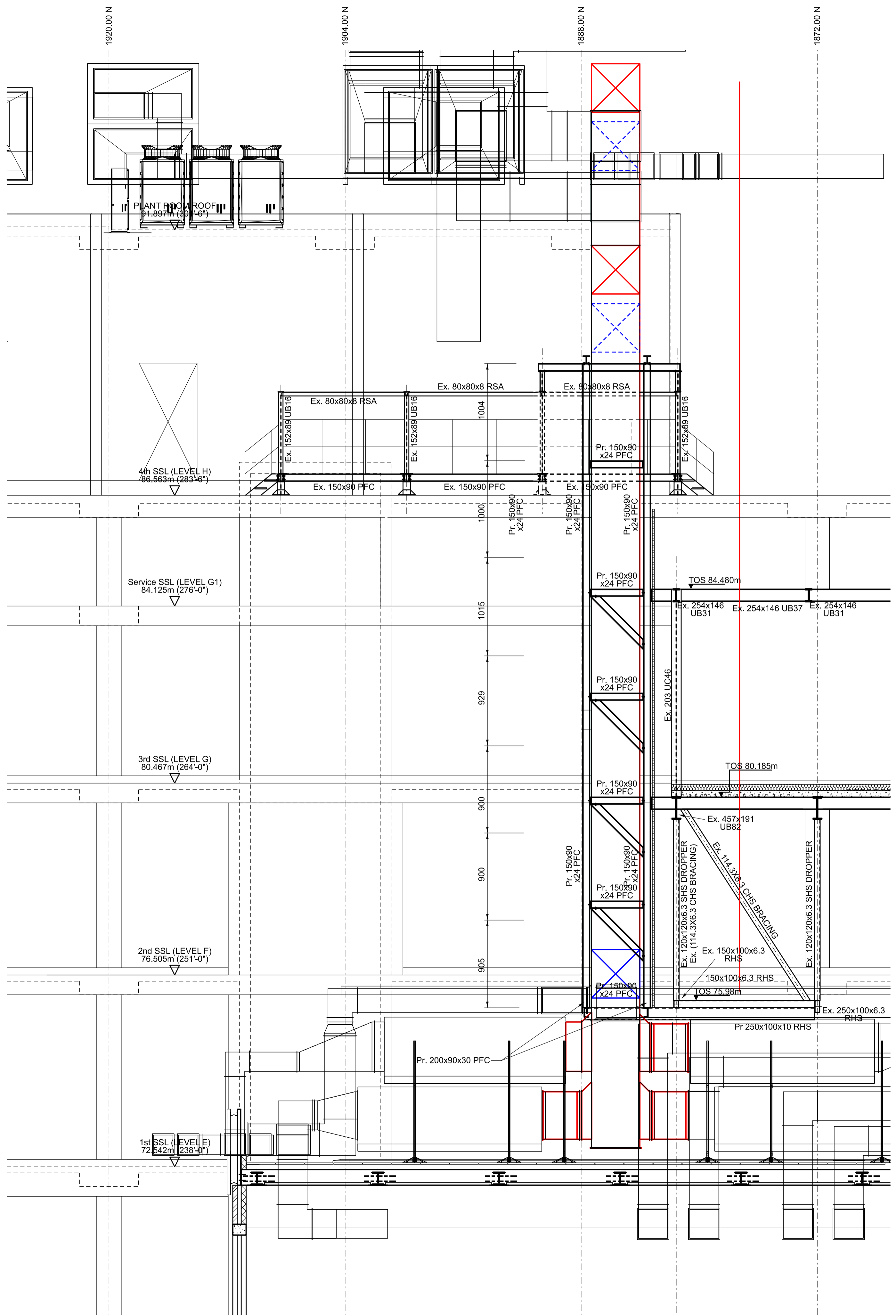
ELEVATION OF RISER
