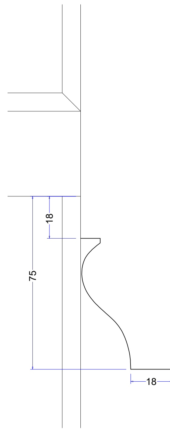
HORN DETAIL Scale: 1:1 @A1
