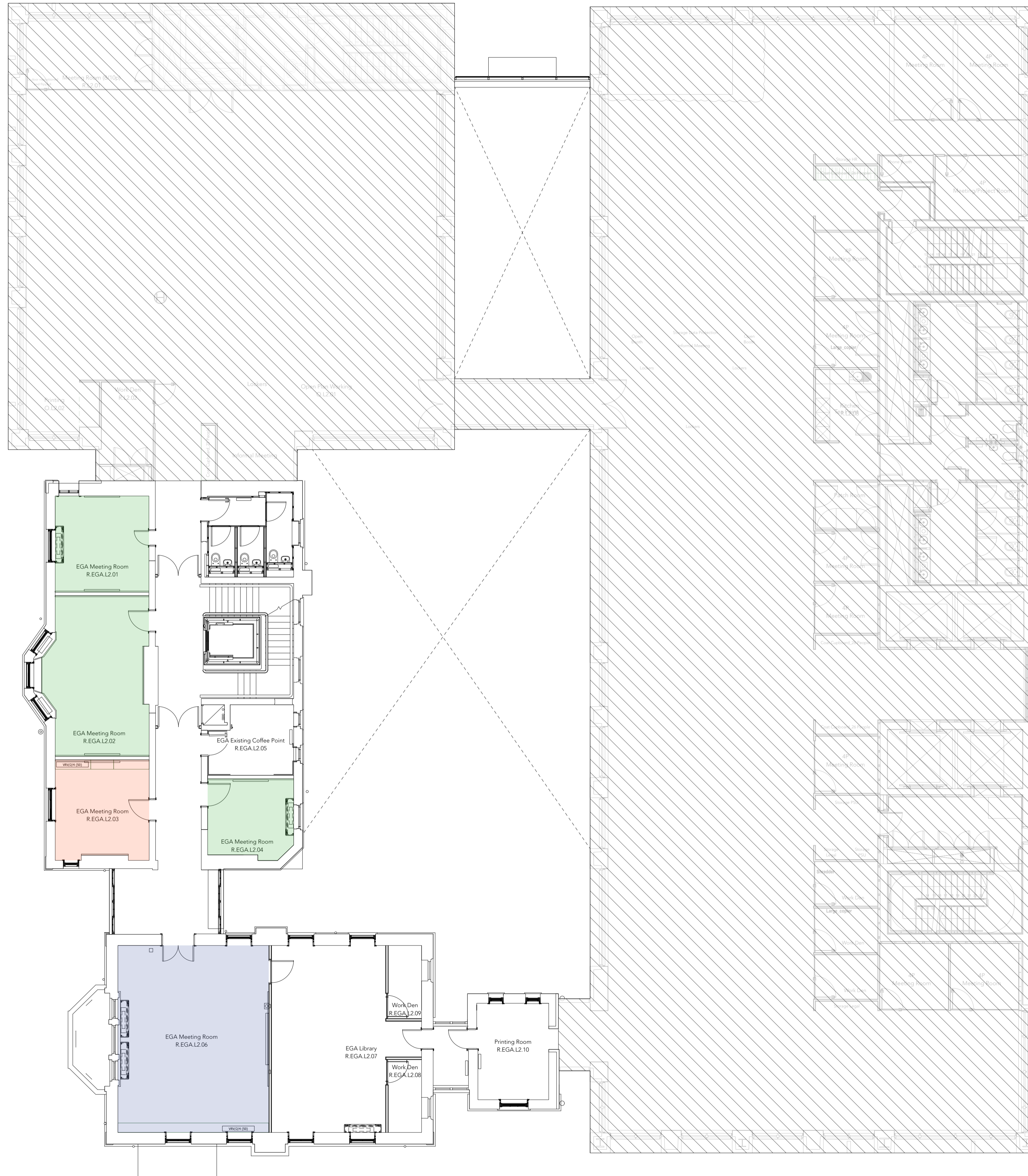
1 Second Floor General Arrangement Scale: 1:100
