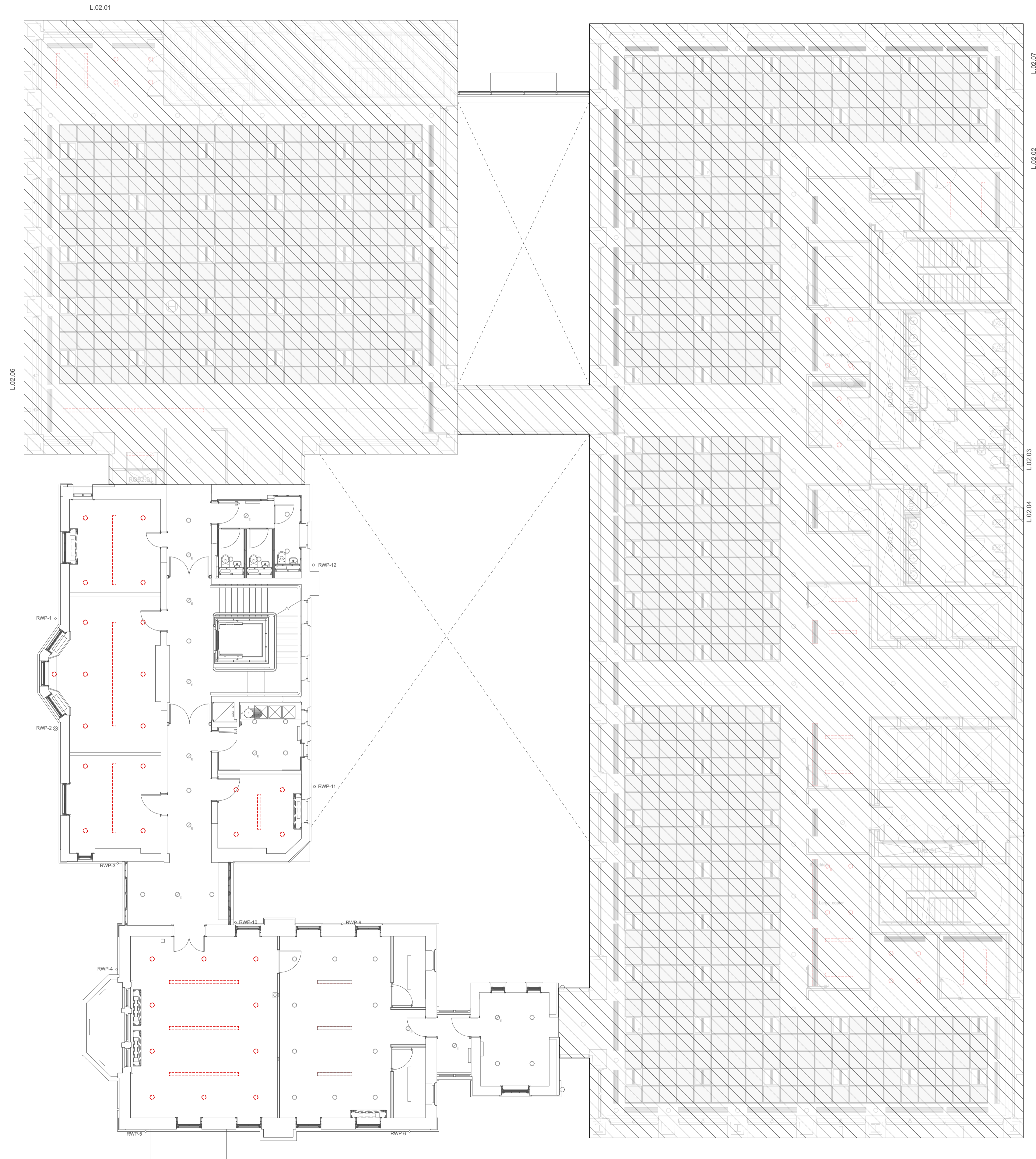
1 Second Floor Demolition Ceiling Scale: 1:100
