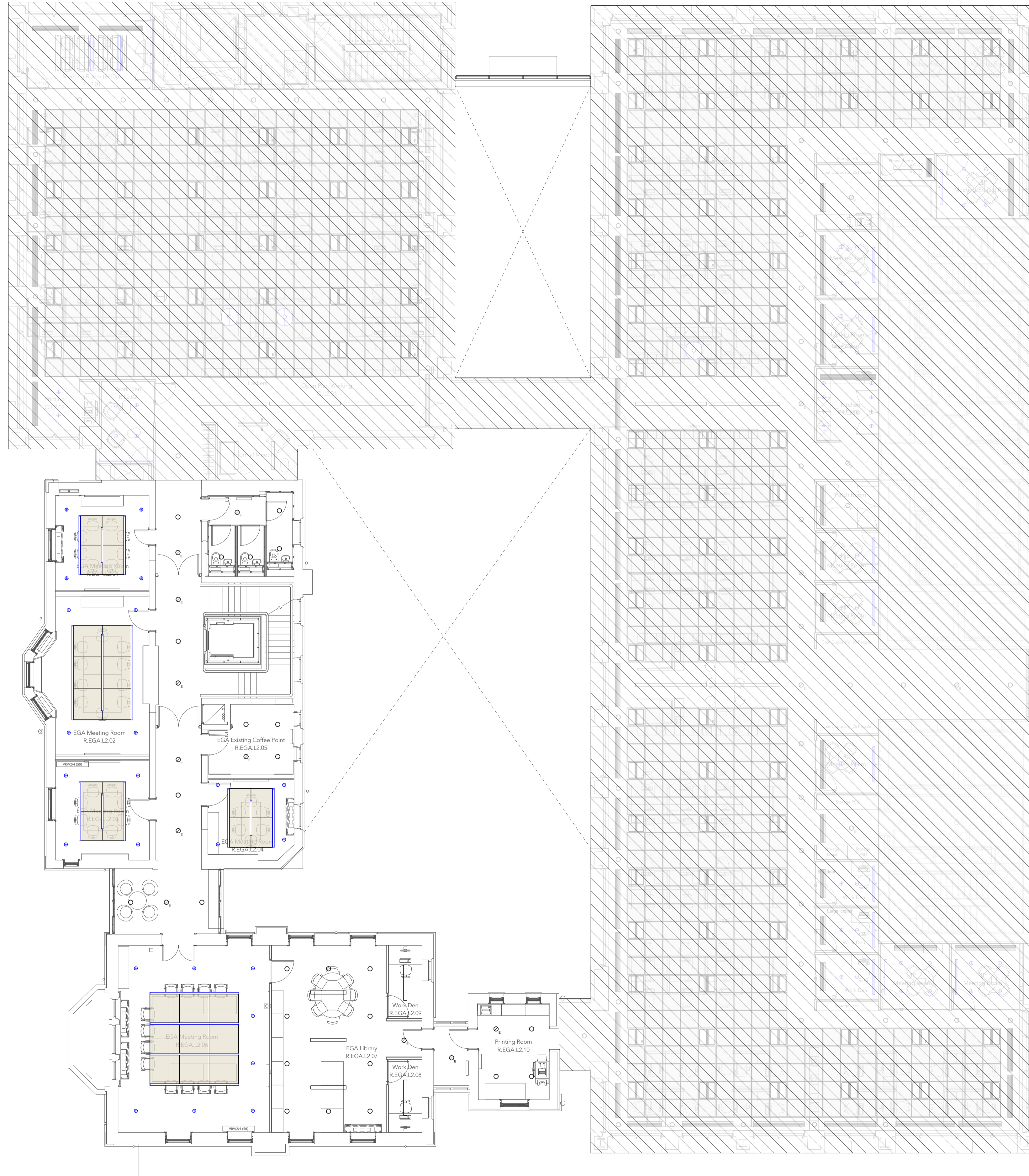
1 Second Floor Proposed Ceiling Arrangement Scale: 1:100
