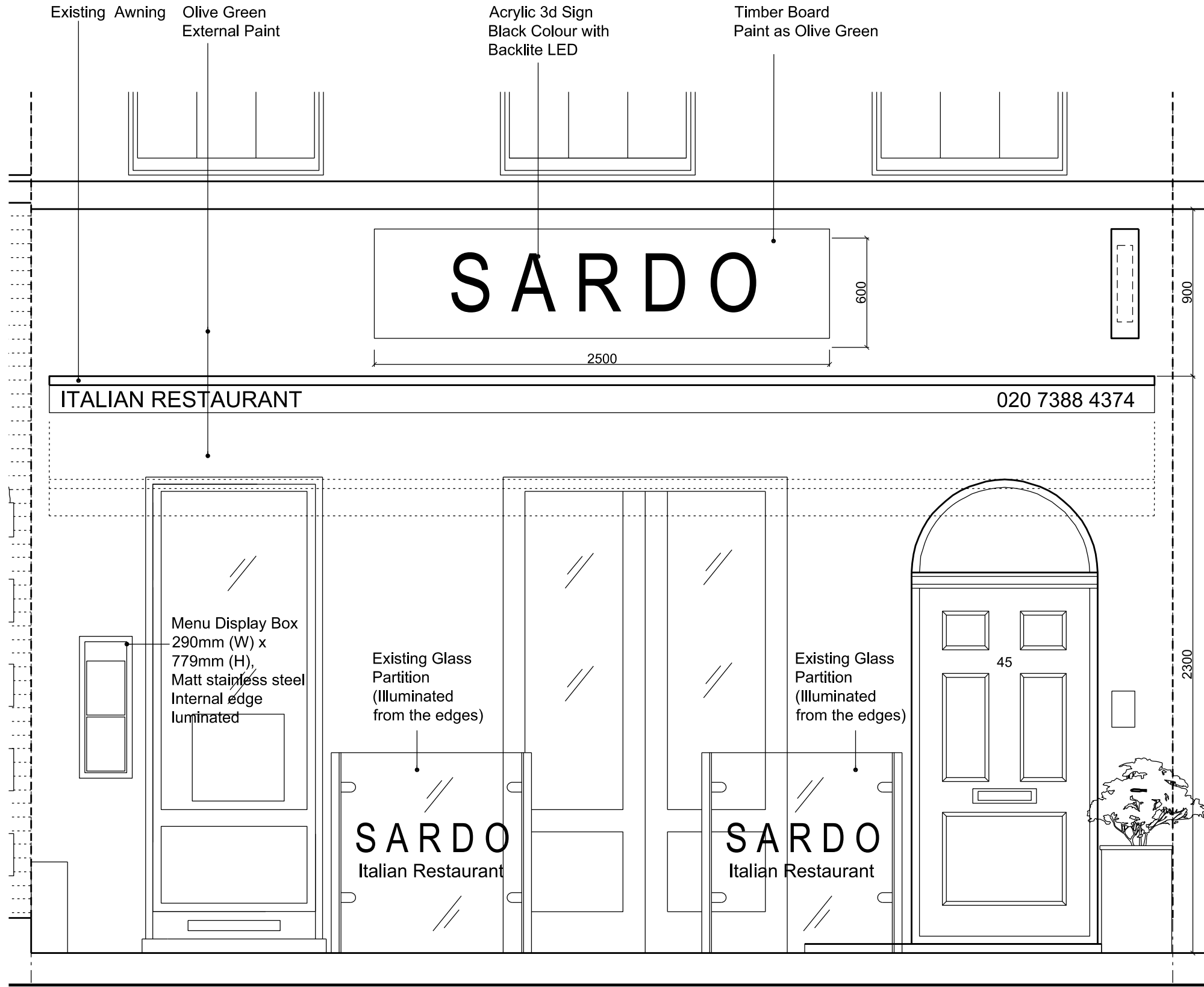
01 EXISTING SHOPFRONT AND ADVERTISEMENT A-E-00 Scale 1:25
