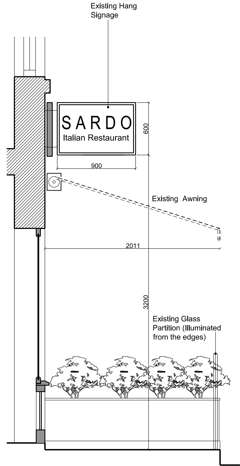
02 SECTION - EXISTING SHOPFRONT A-E-00 Scale 1:25
