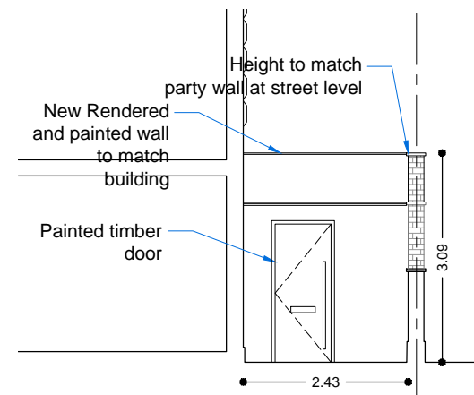
3_Stairs elevation
