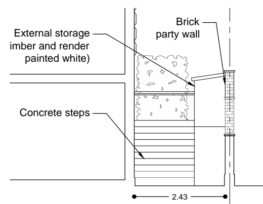
3_Stairs elevation
