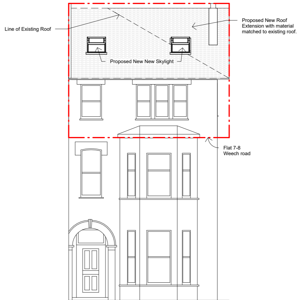
Proposed Front Building Elevation
