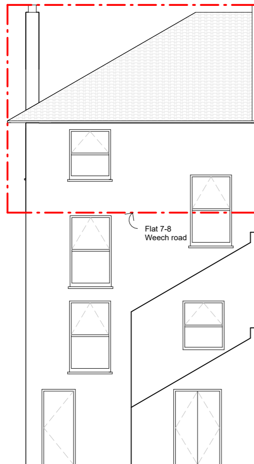
Existing Rear Building Elevation
