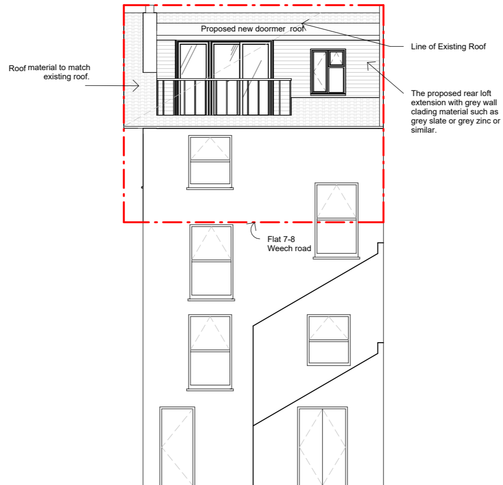
Proposed Rear Building Elevation
