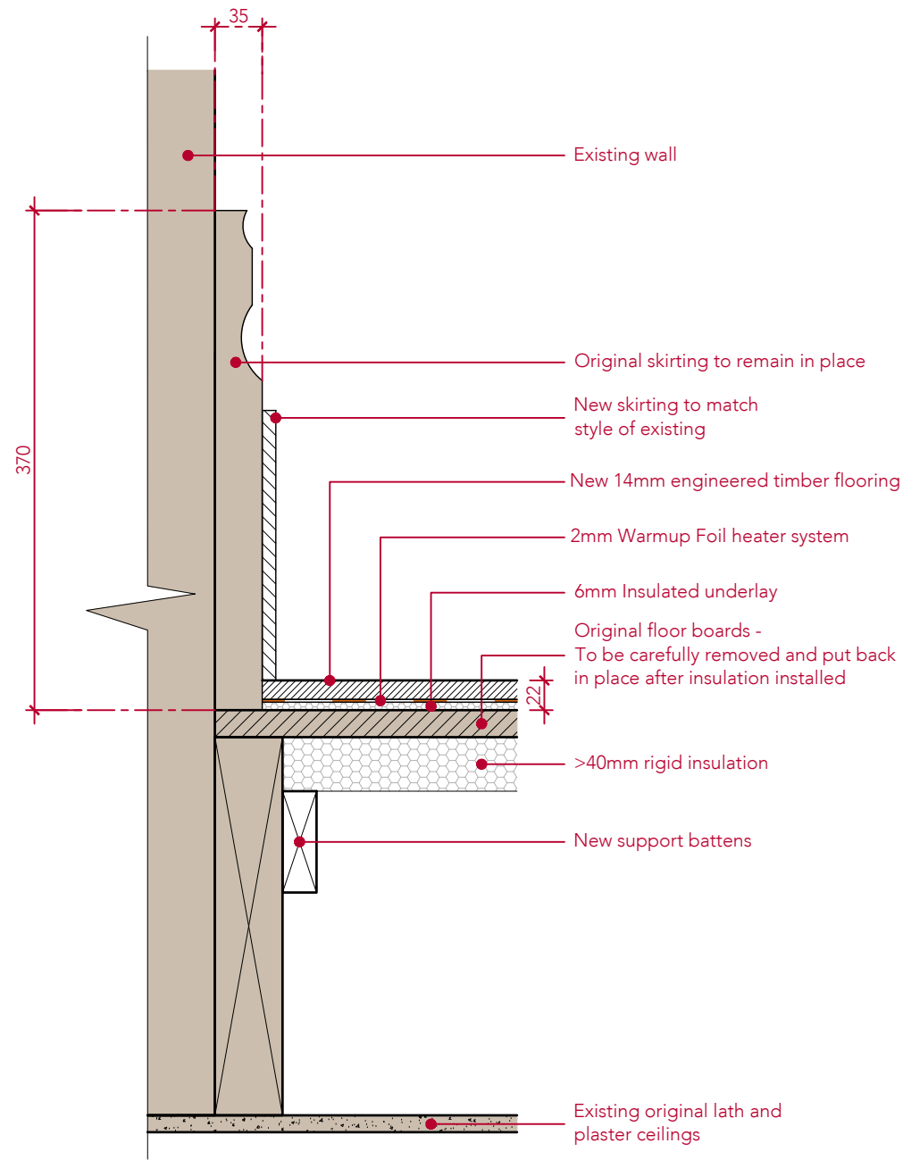
1 GF FLOOR/SKIRTING BUILDUP scale 1:5
