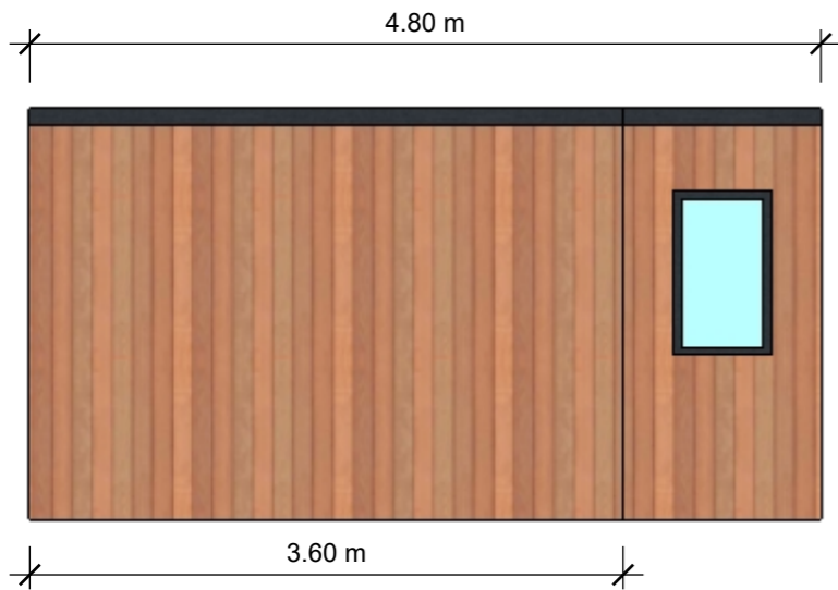
West Elevation
