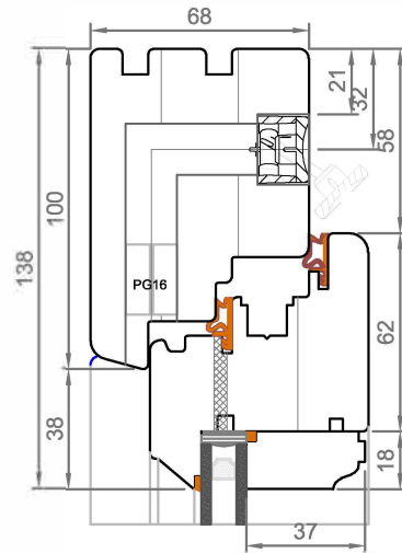
HEAD DETAIL WINDOW REF: Side1, Side2
