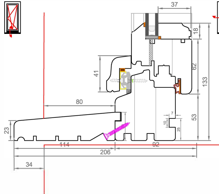
CILL DETAIL WINDOW REF: Side1, Side2
