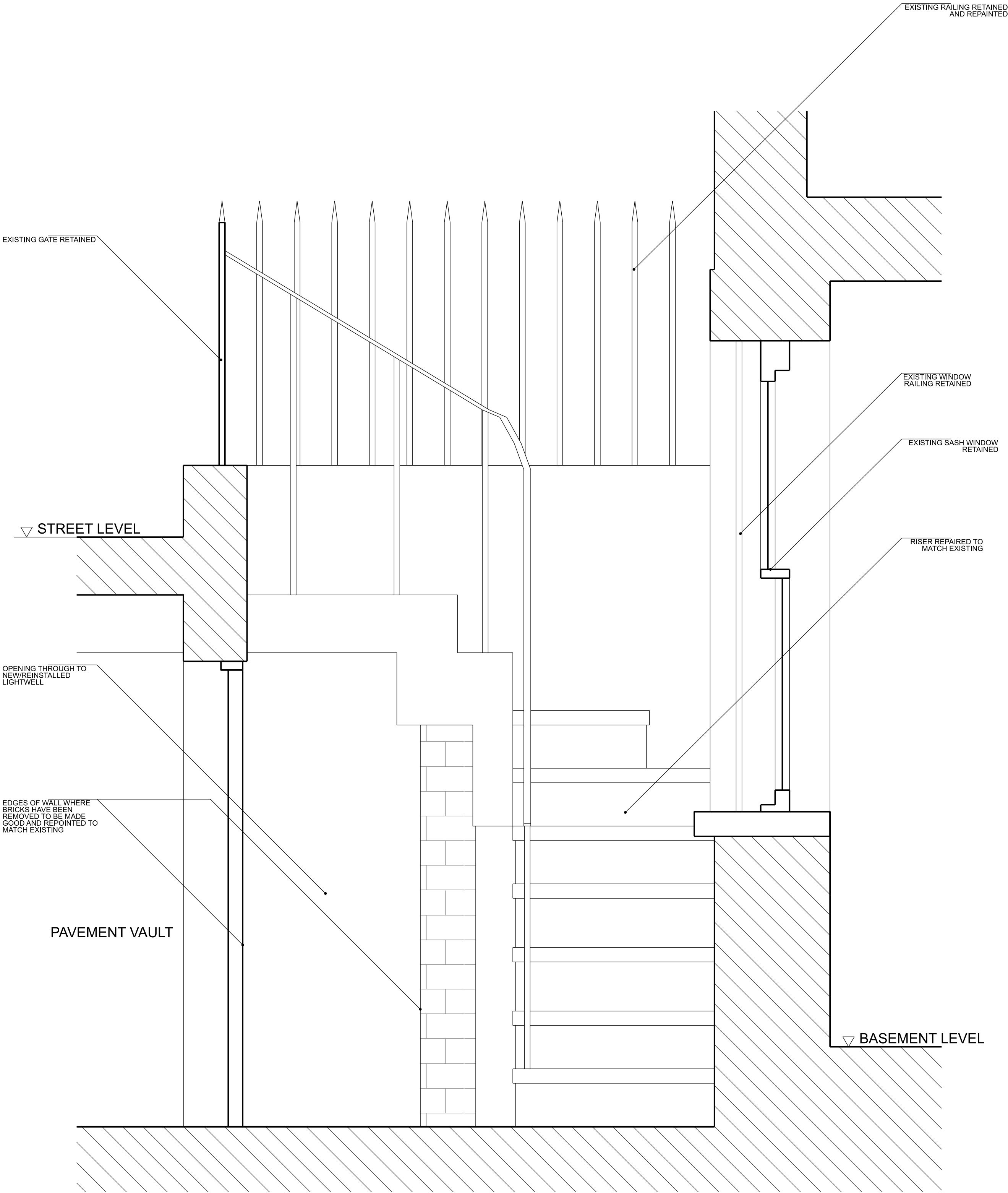
2 1:10@ A1, 1:20@ A3 PROPOSED LIGHTWELL SECTION
