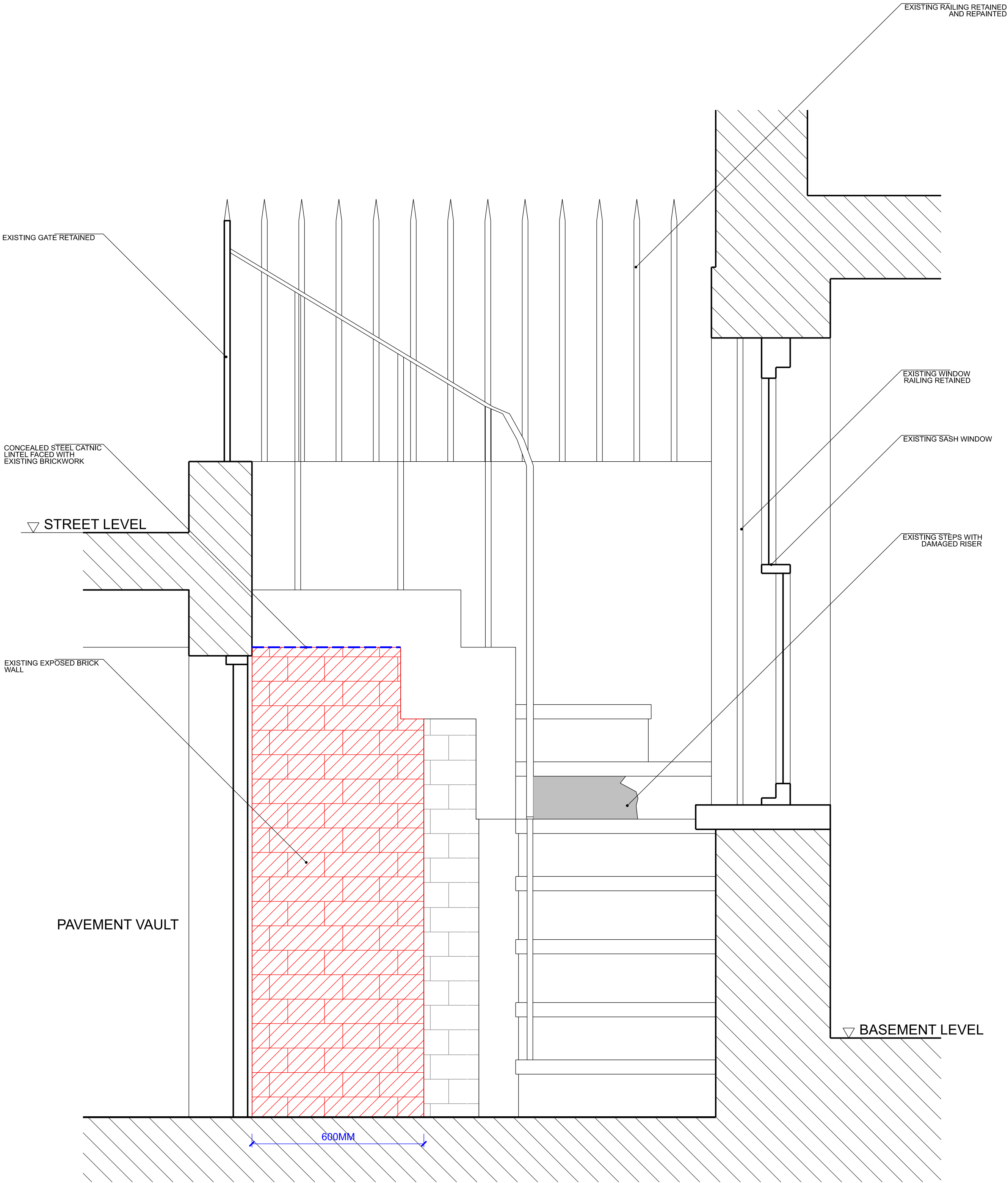
1 1:10@ A1, 1:20@ A3 EXISTING LIGHTWELL SECTION WITH ALTERATION
