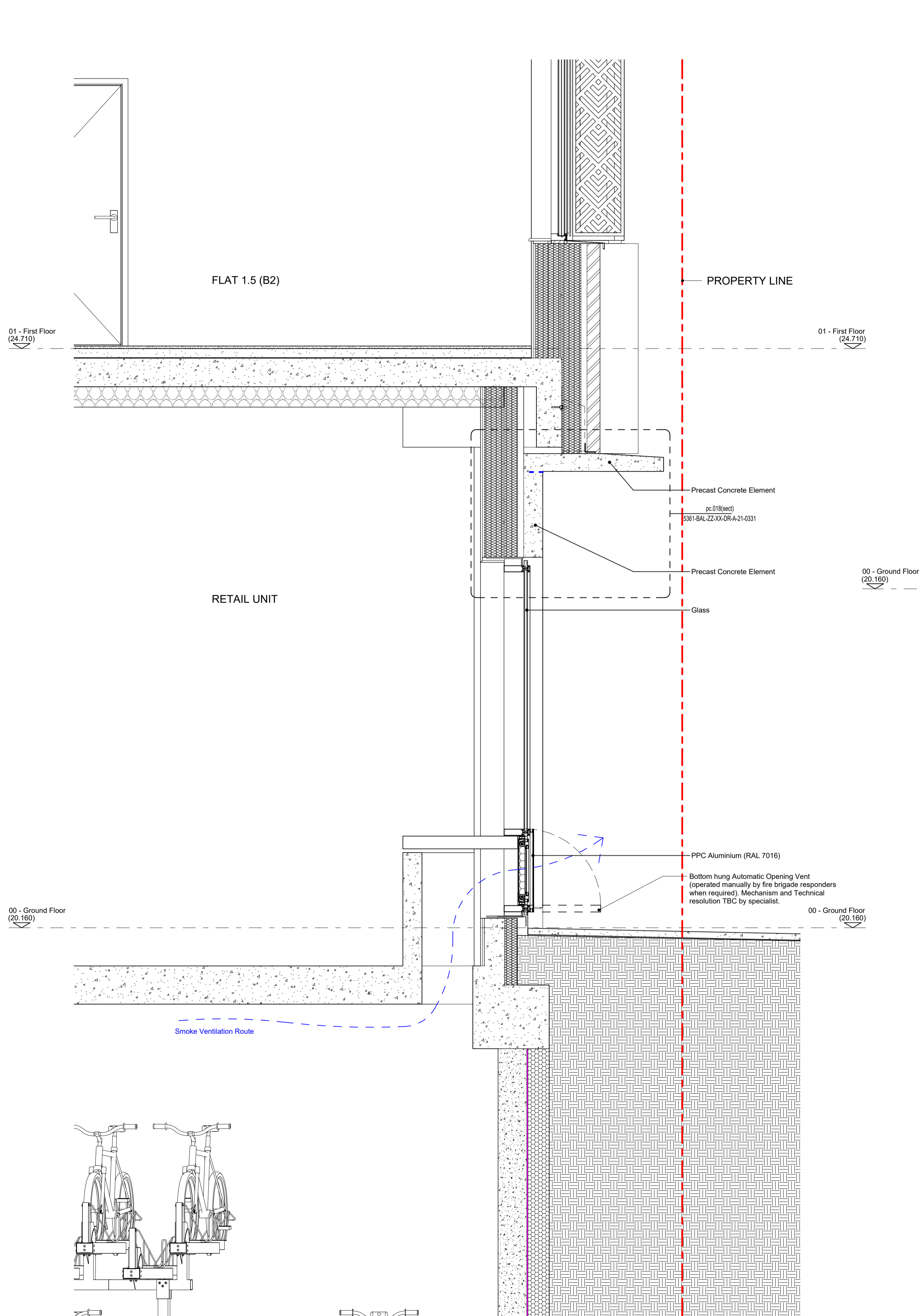
os.C.01 - Section C - Retail Unit (Smoke Vent) - Gray's Inn Rd 1 : 20
