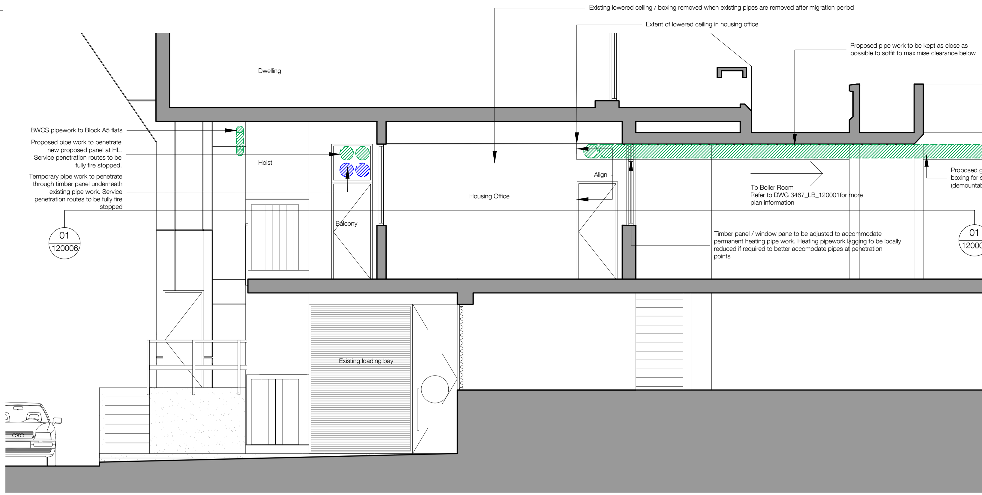
01 Block A - Section A Through Housing Office Temporary and Final Condition - 1:50
