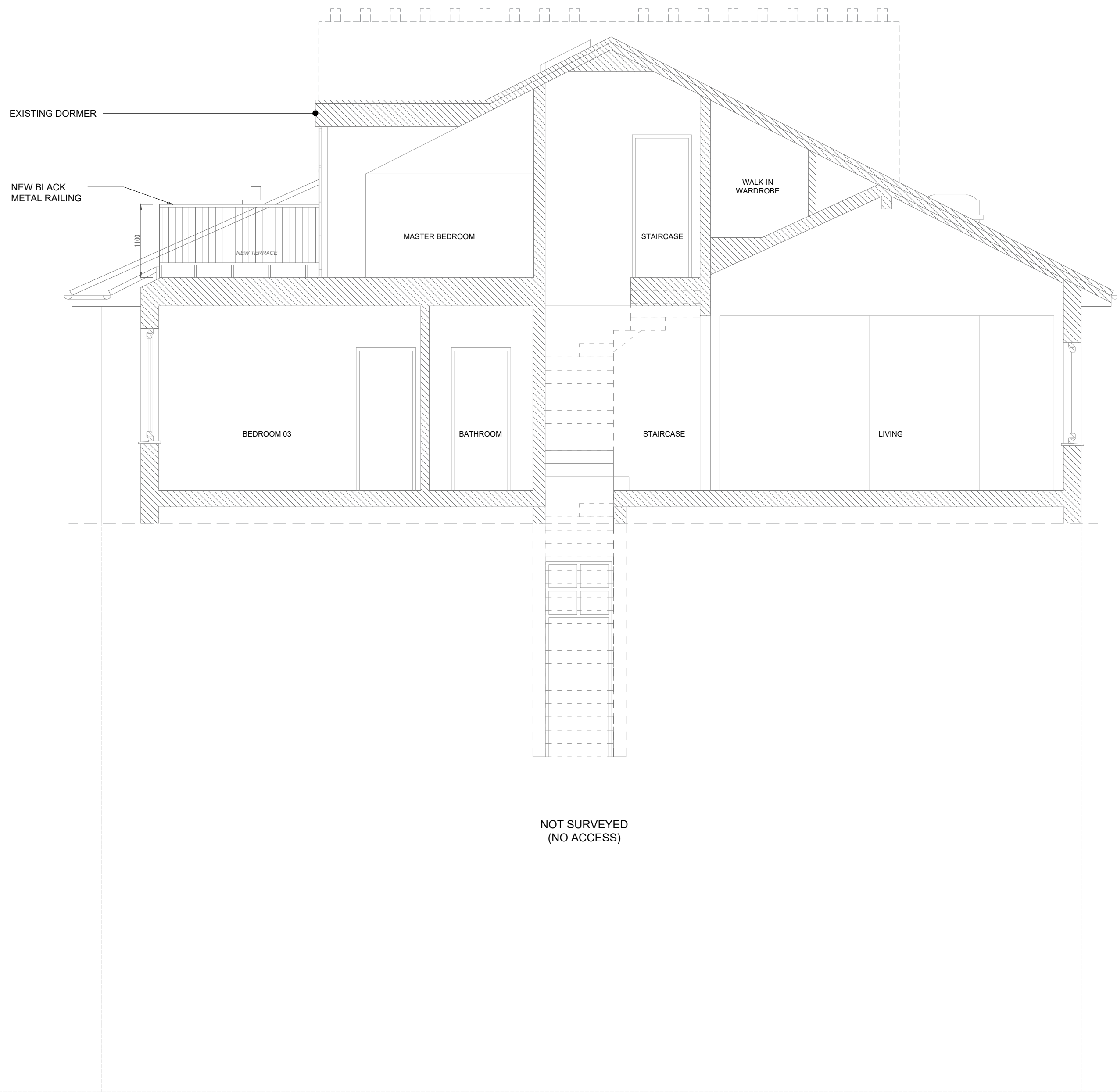
SECTION A-A (1:50)
