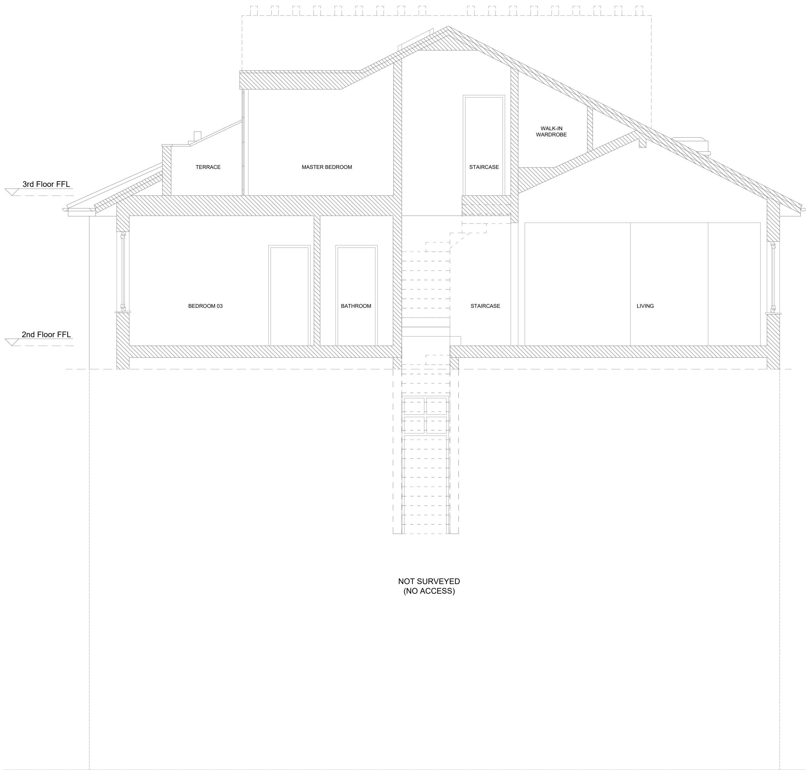
SECTION A-A (1:50)
