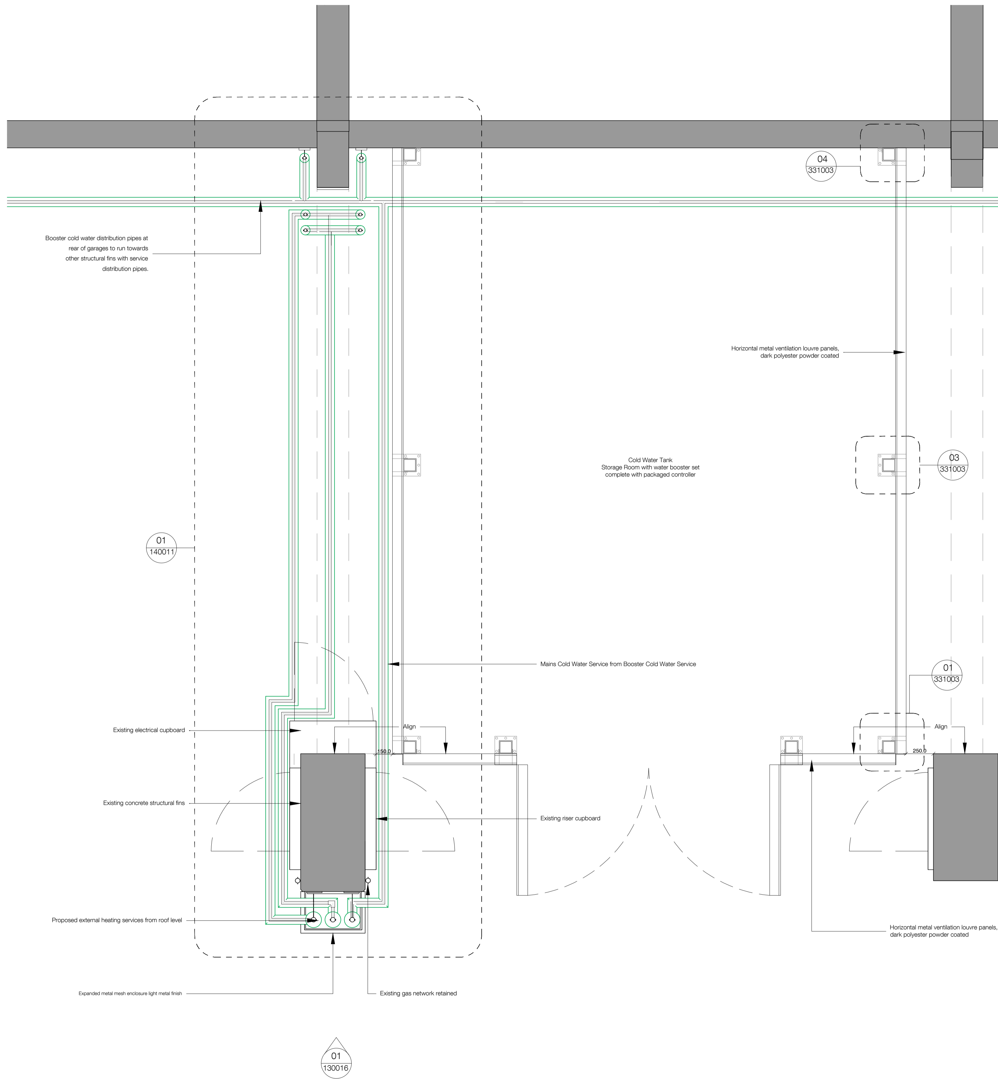
01 Block A - Cold Water Storage Tank Plan 1:20
