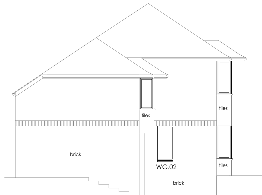
WEST ELEVATION
