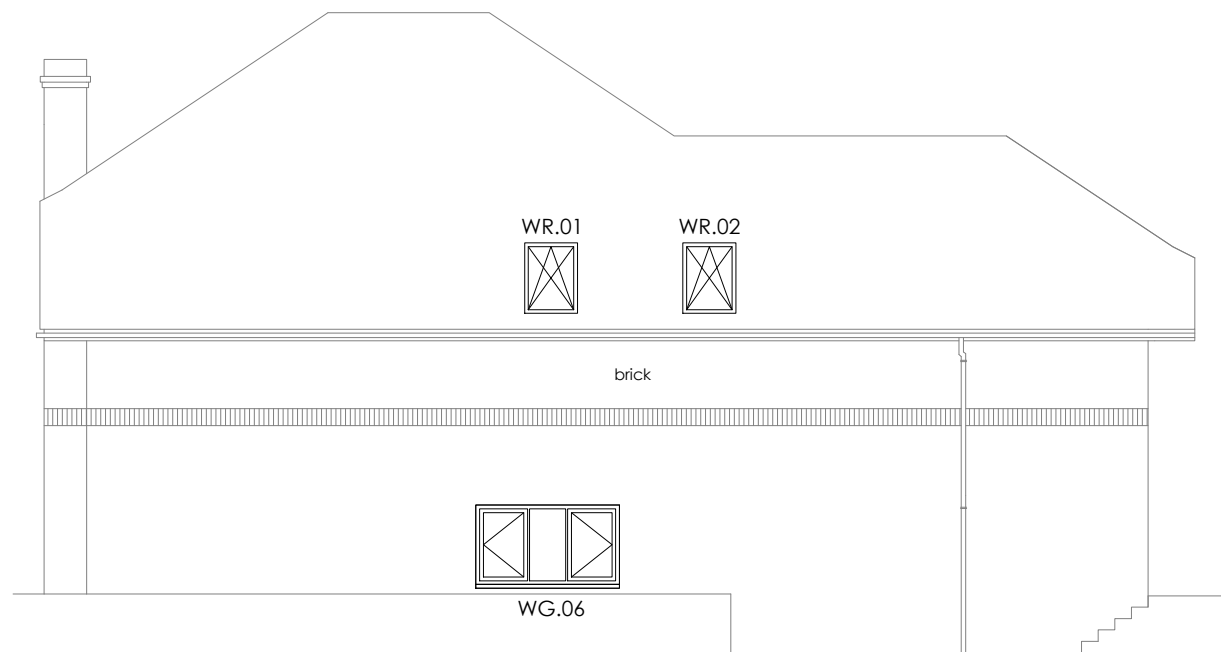
NORTH ELEVATION
