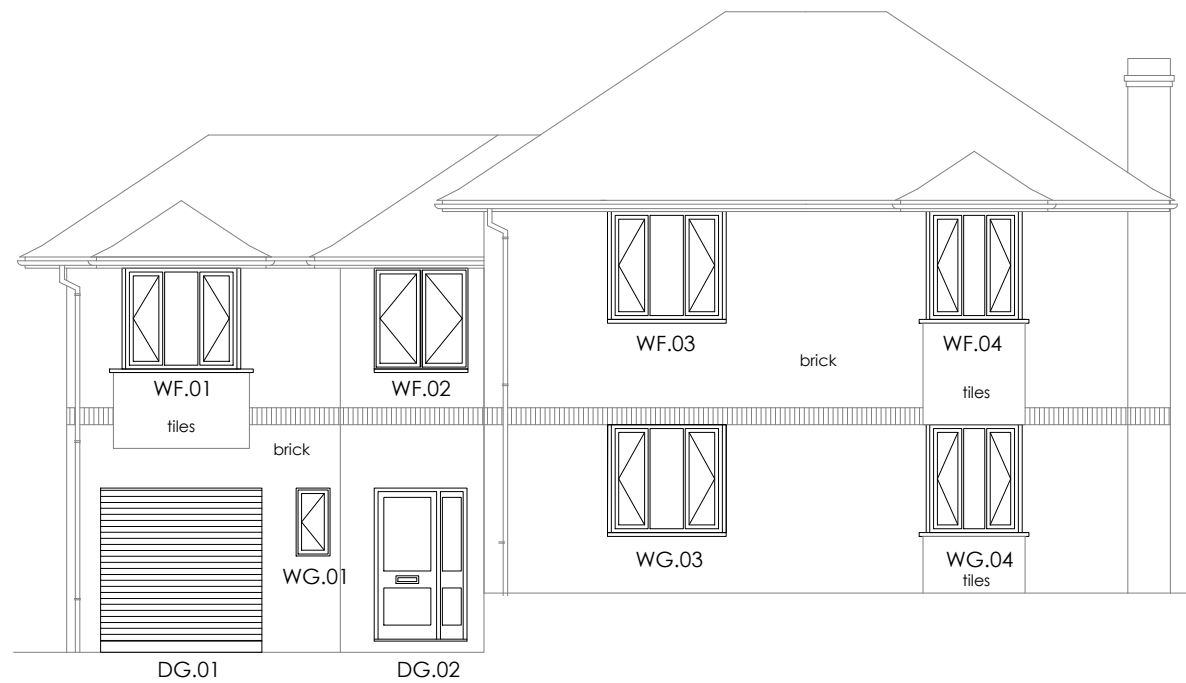
SOUTH ELEVATION
