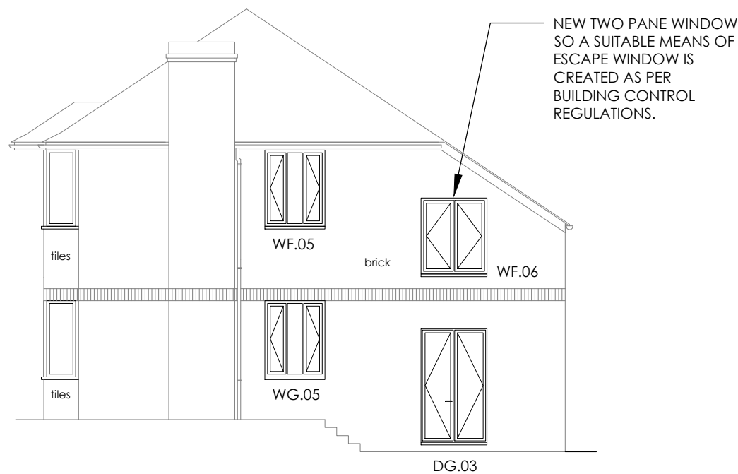
EAST ELEVATION
