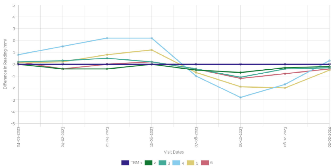
Level Readings Chart (Points TBM 1 - 6)
