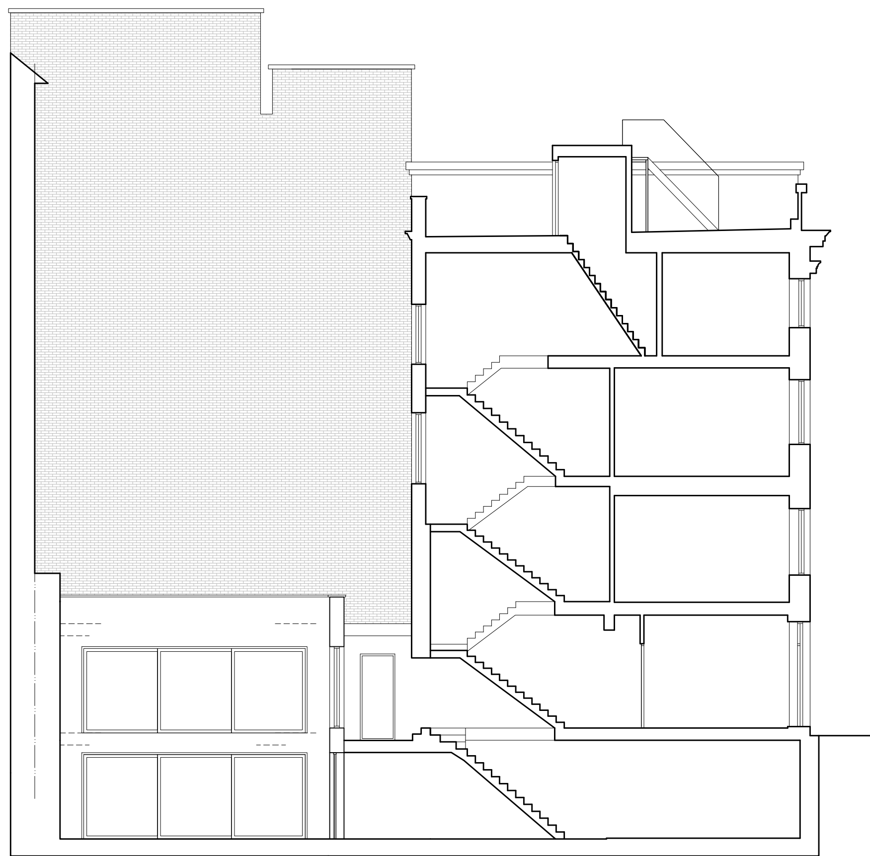
Proposed East Elev/Section Scale 1:100
