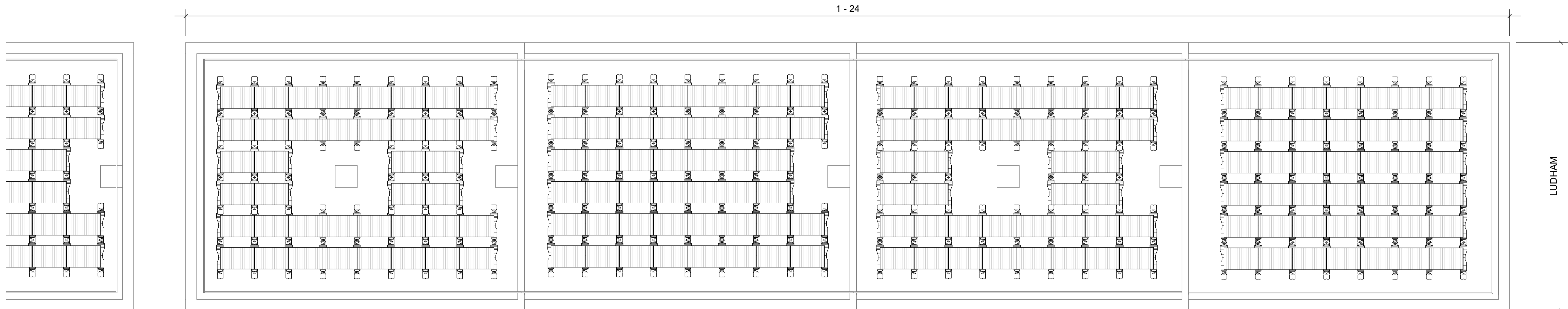
1 Proposed Roof Plan - Sheet 4 1 : 100
