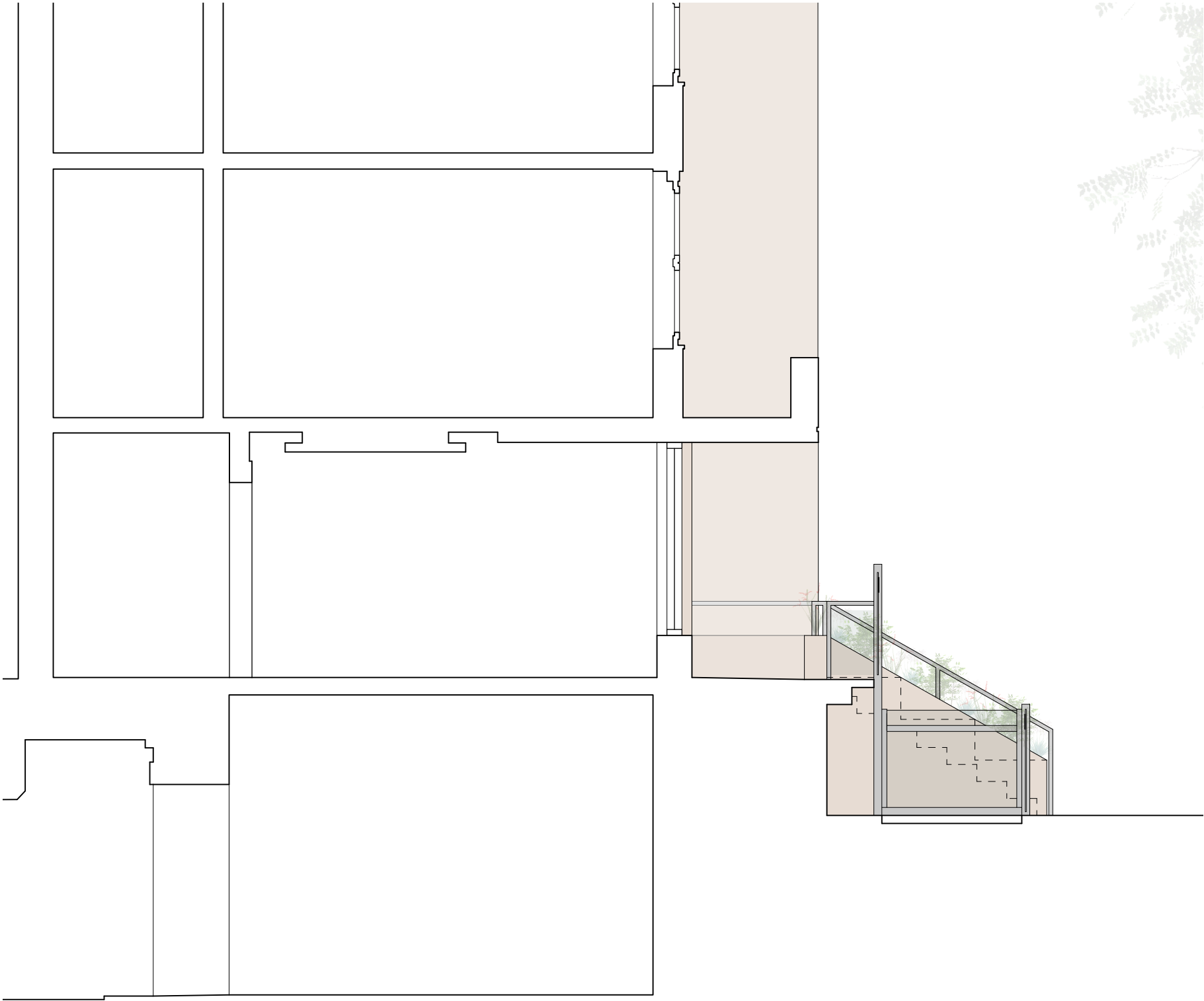
Proposed Level Access Platform Lift Section
