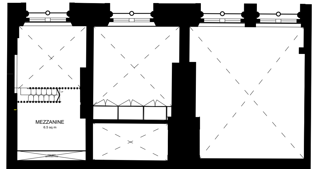
4 PROPOSED MEZZANINE PLAN SCALE 1:100@A3
