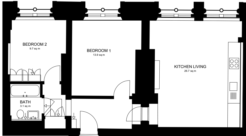
1 EXISTING PLAN SCALE 1:100@A3
