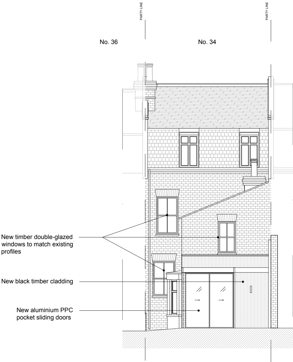
PROPOSED REAR FACADE Scale 1:100@A3
