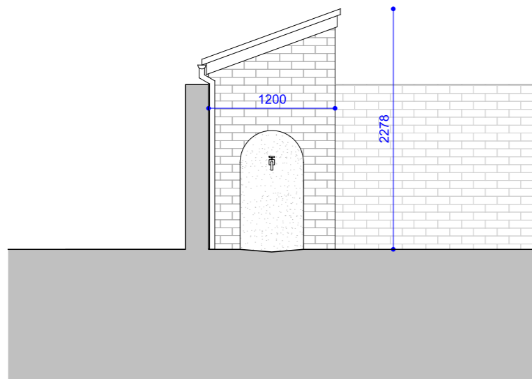
02. Garden Store Side Elevation
