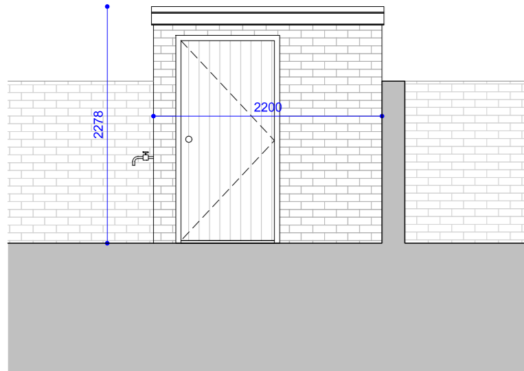
01. Garden Store Front Elevation
