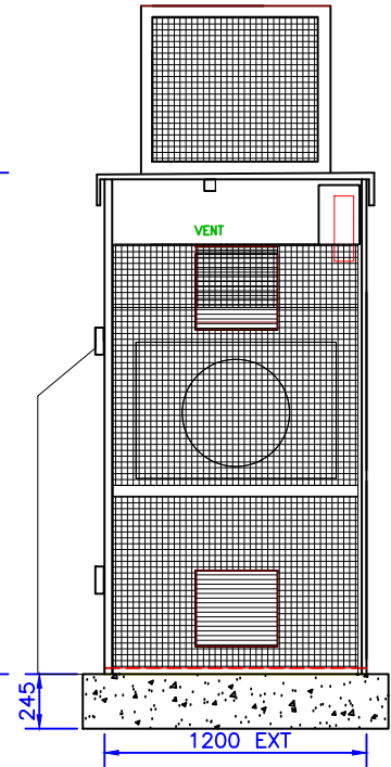
END VIEW 2
