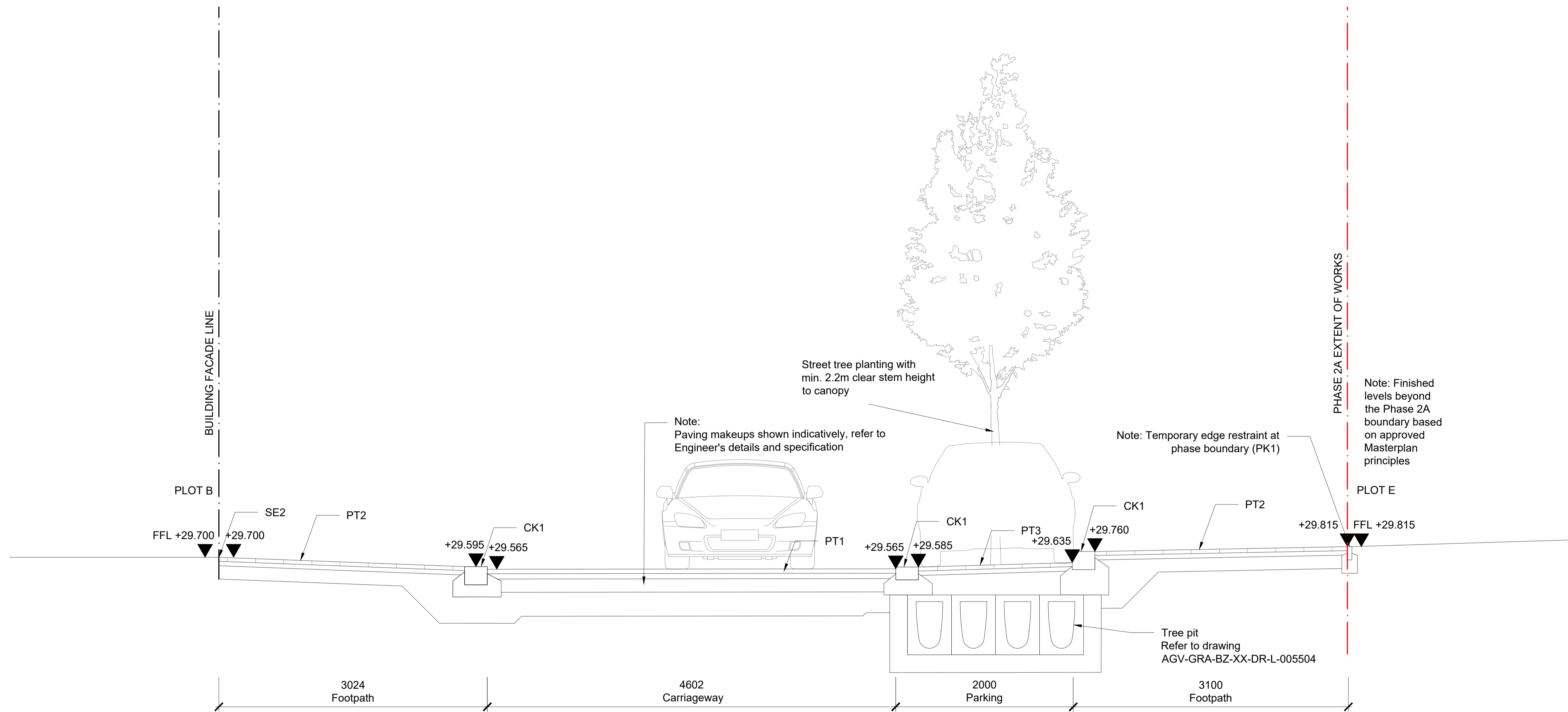
C-C Cross Section through Wrotham Road (West) scale 1:25 @ A1
