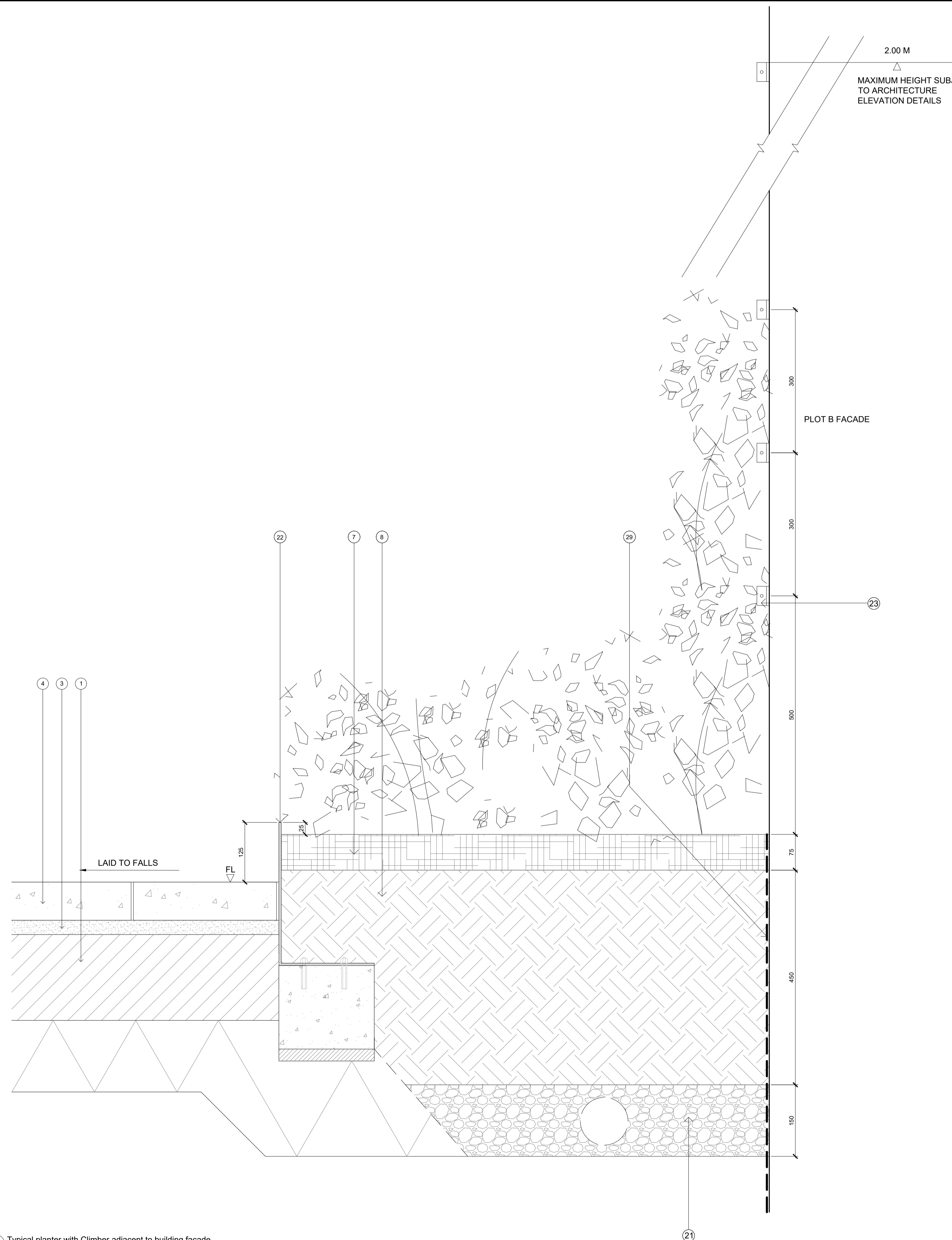
1 Typical planter with Climber adjacent to building façade SCALE 1:5
