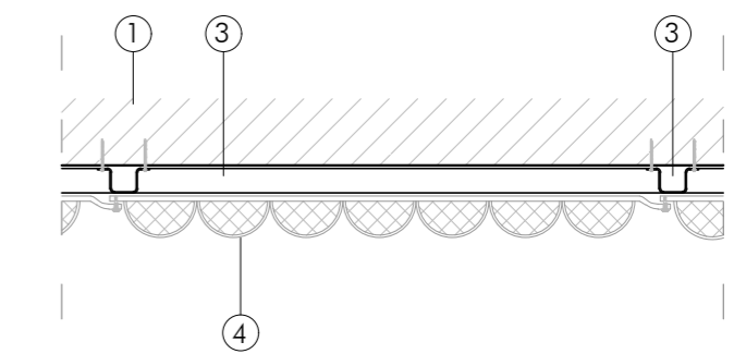
DETAILED HORIZONTAL SECTION
