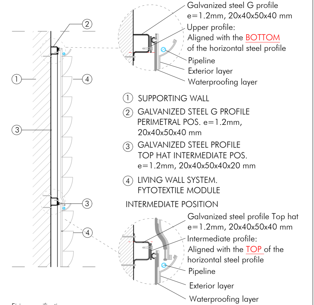
Fixing specifications:
