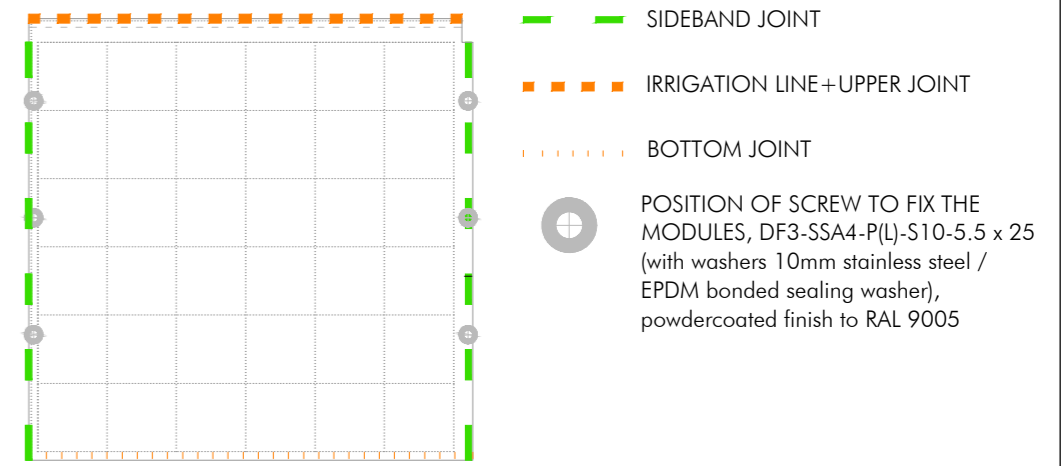
PERIMETER SCREW FOR FYTOTEXTILE 36 MODULES
