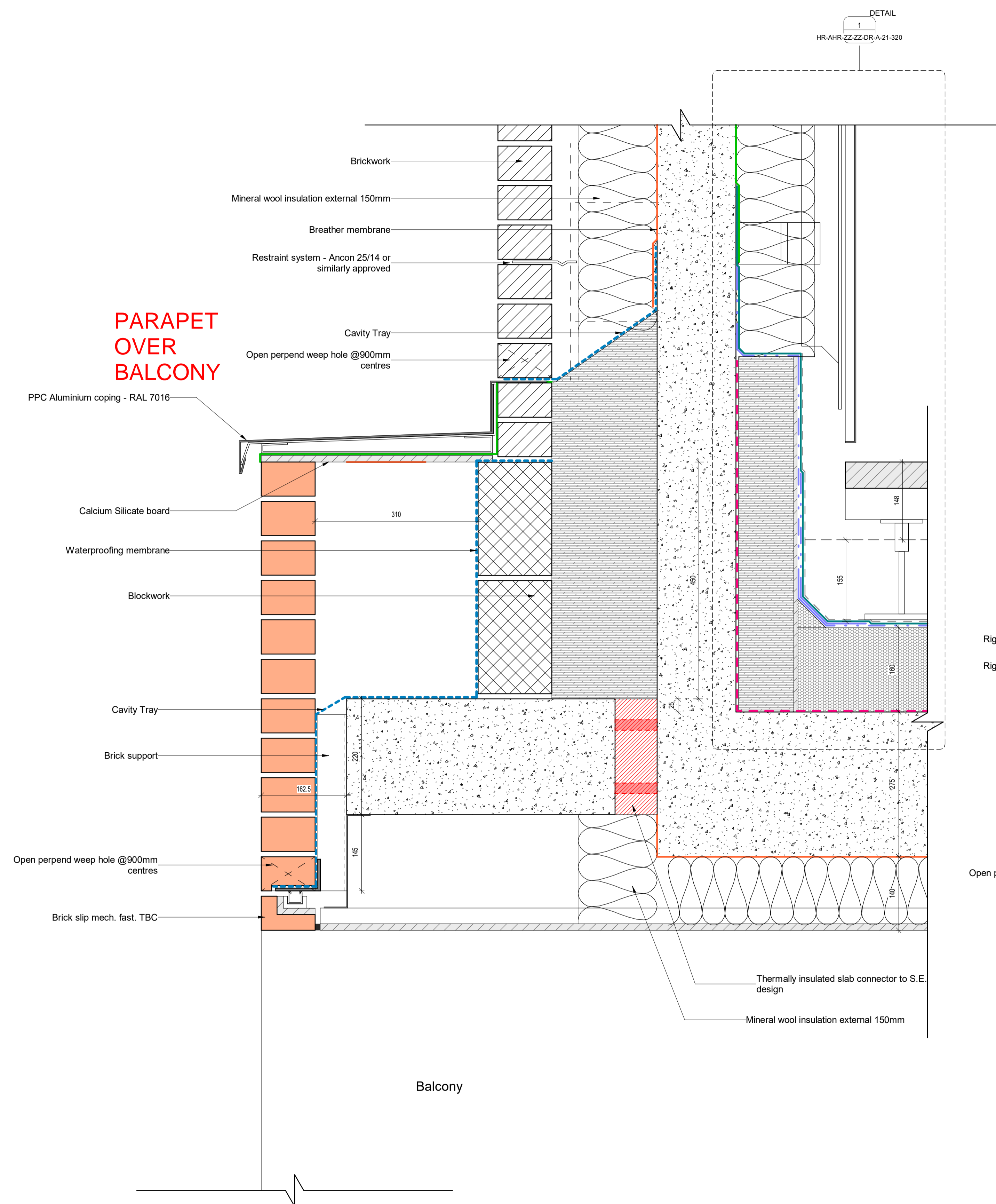
1 Typical Detail Roof over Balcony 1 : 5
