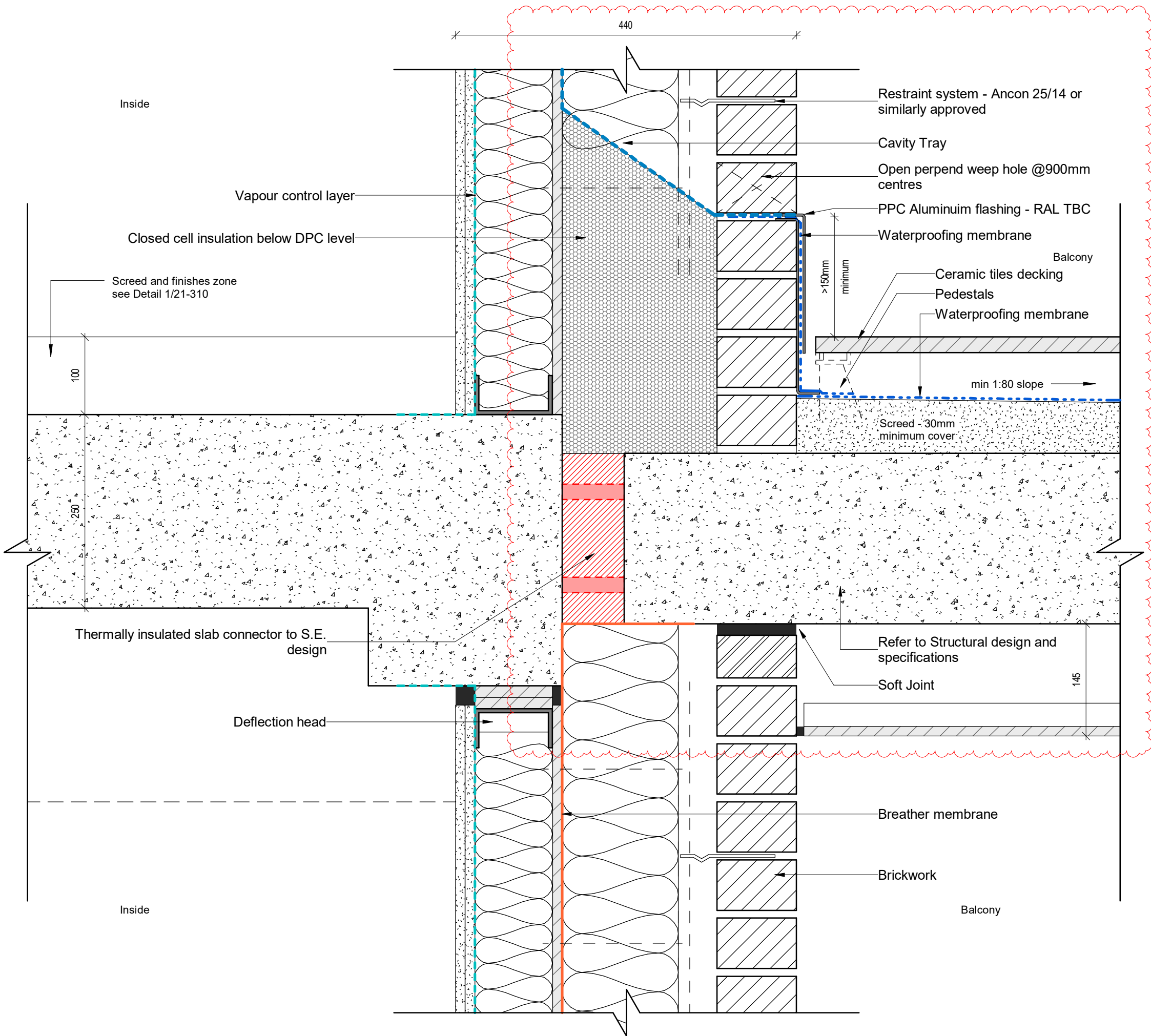
A Typical Detail Balcony A 1:5
