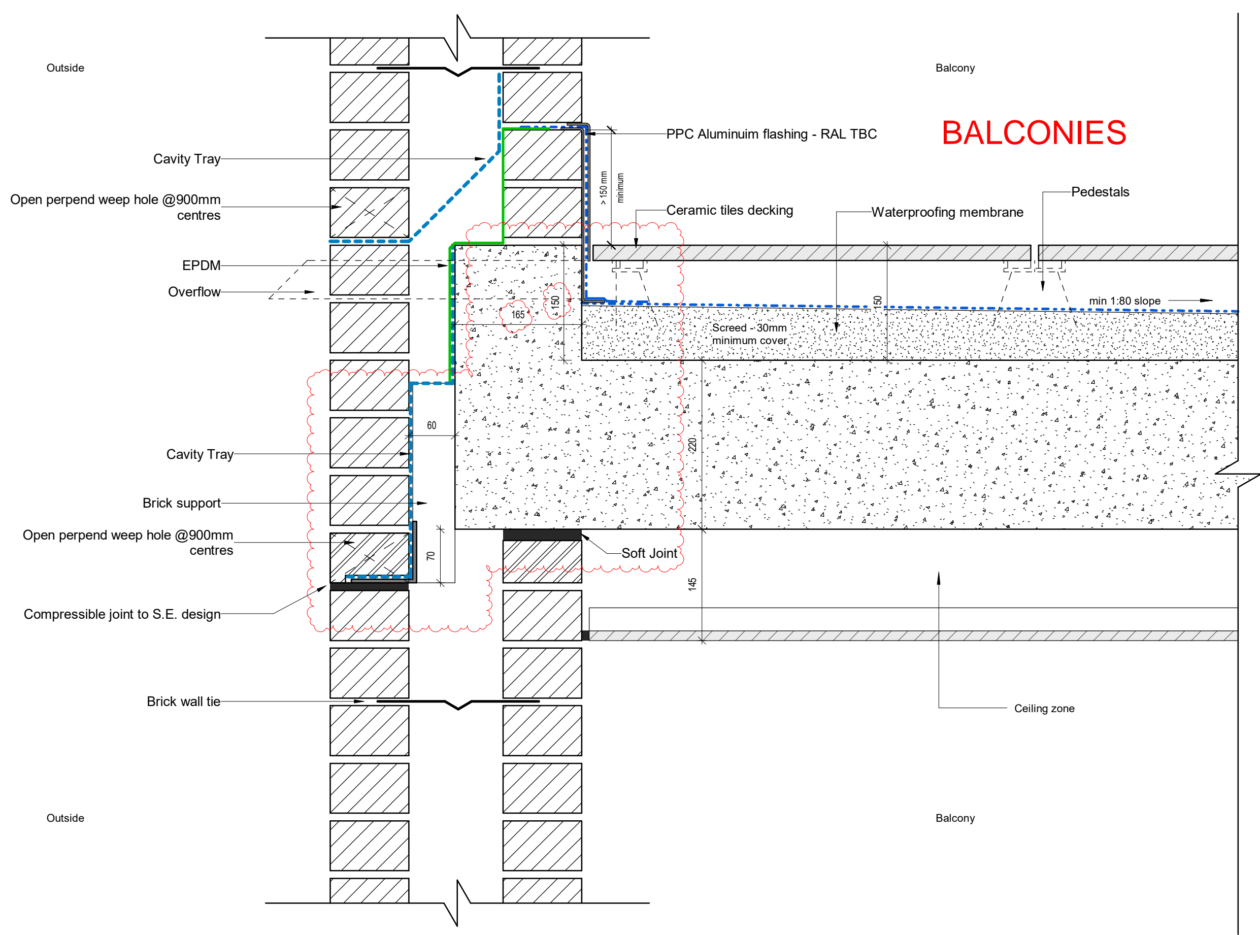
B Typical Detail Balcony B 1:5
