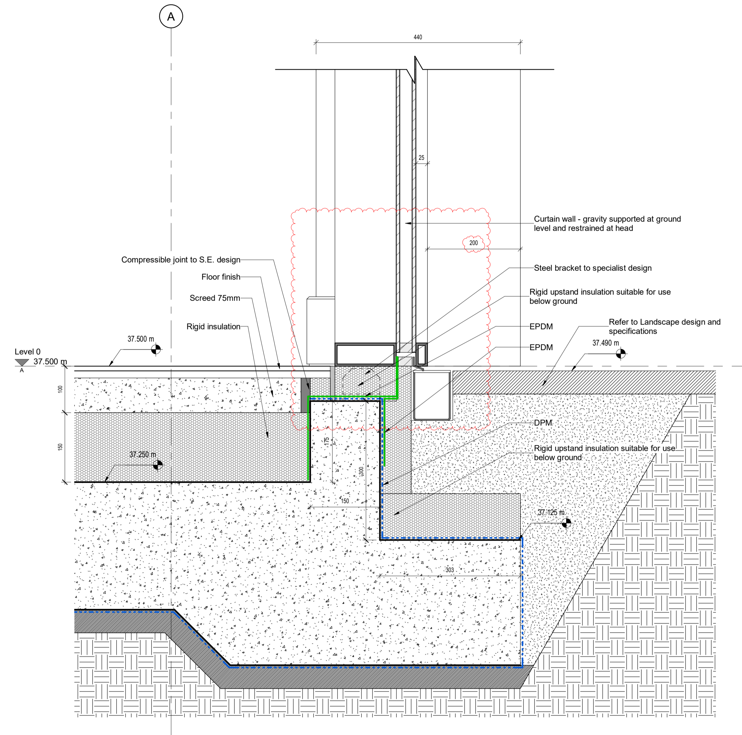
2 GF Section 2 Detail 1-5 1:5
