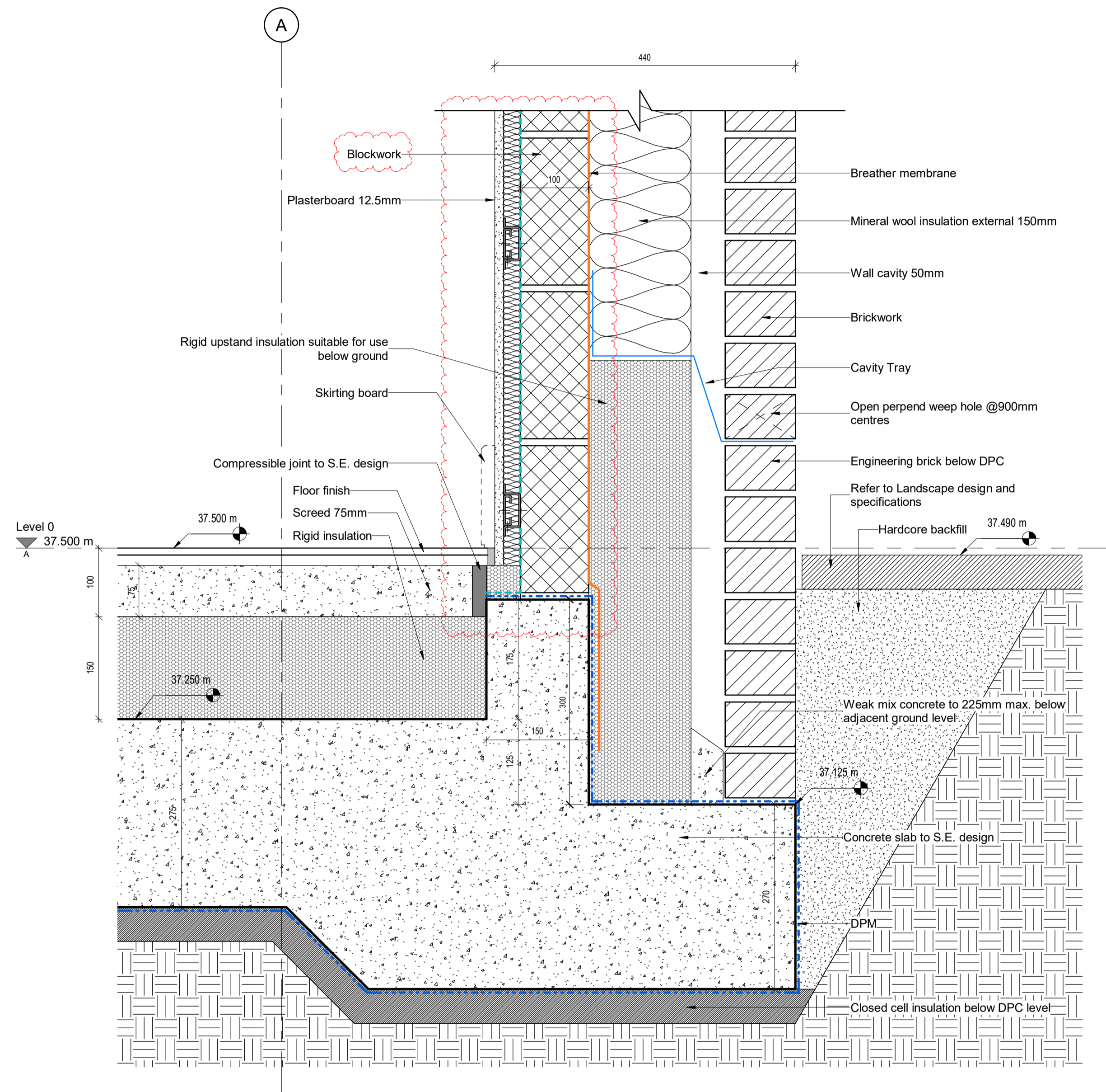
1 GF Section 1 Detail 1-5 1:5
