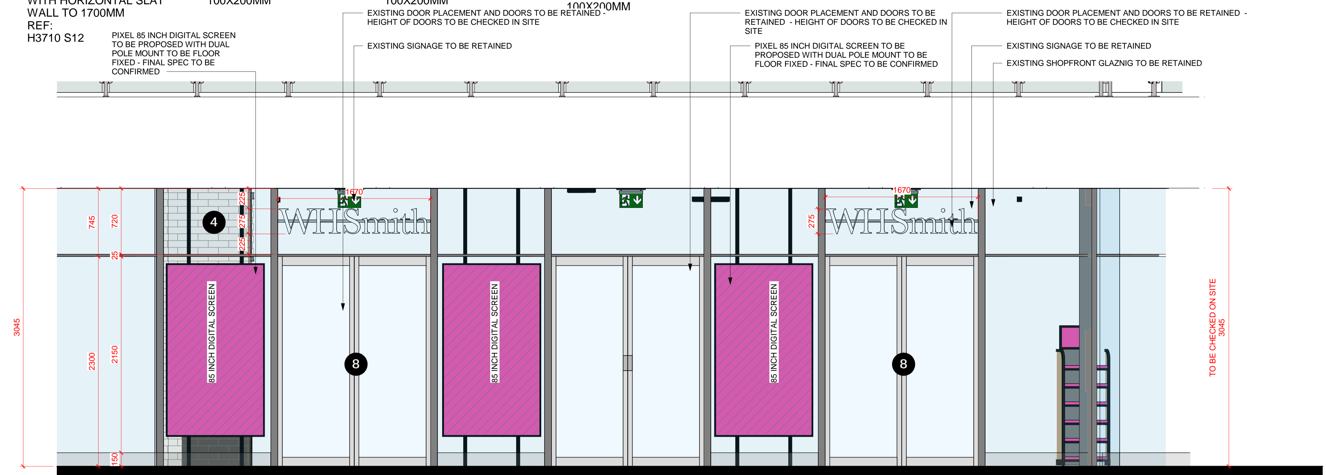
1 EXTERNAL ELEVATION 1 1 : 25
