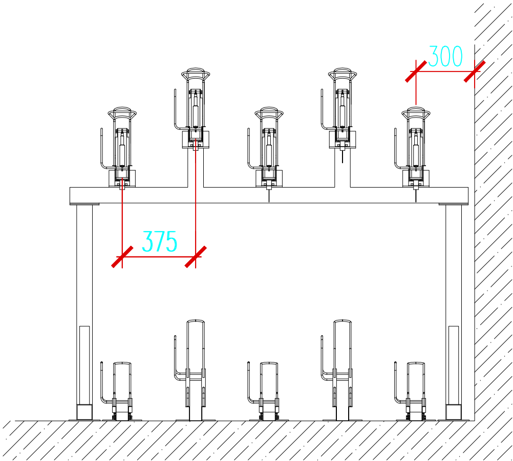
2 TIER RACK ELEVATION
