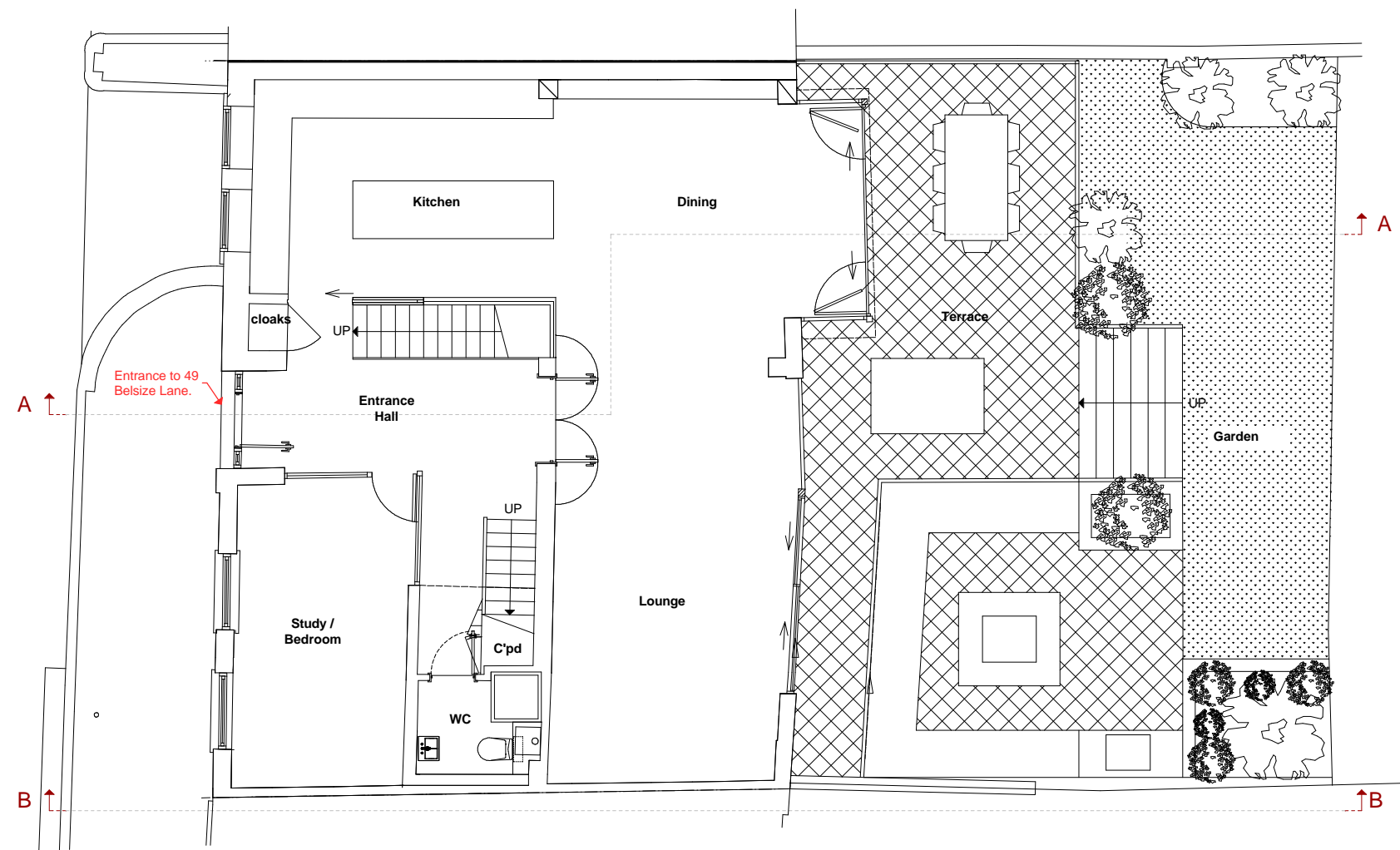
AS-APPROVED GROUND FLOOR PLAN
