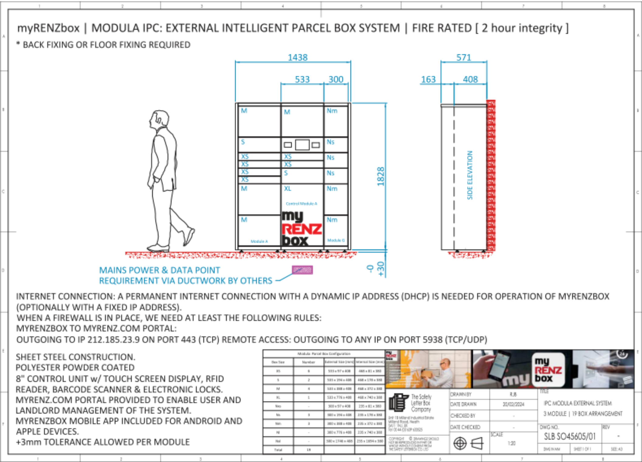
PROPOSED ELEVATION: myRENZbox - External Intelligent Modula Parcel System
