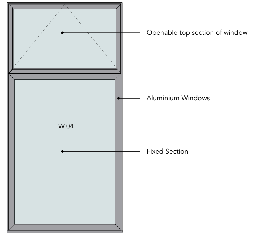
TYPICAL WINDOW ELEVATION
