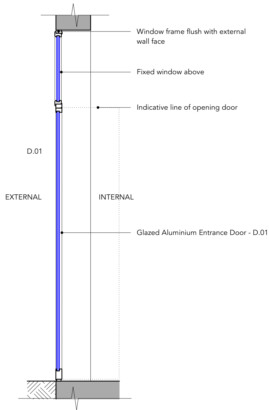
DETAIL 1 - GLAZED ENTRANCE DOOR & FIXED WINDOW
