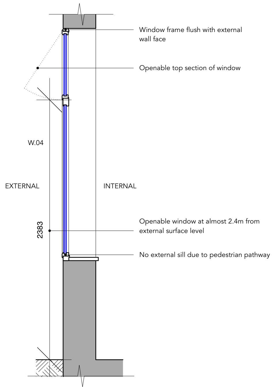
DETAIL 2 - TYPICAL WINDOW SECTION
