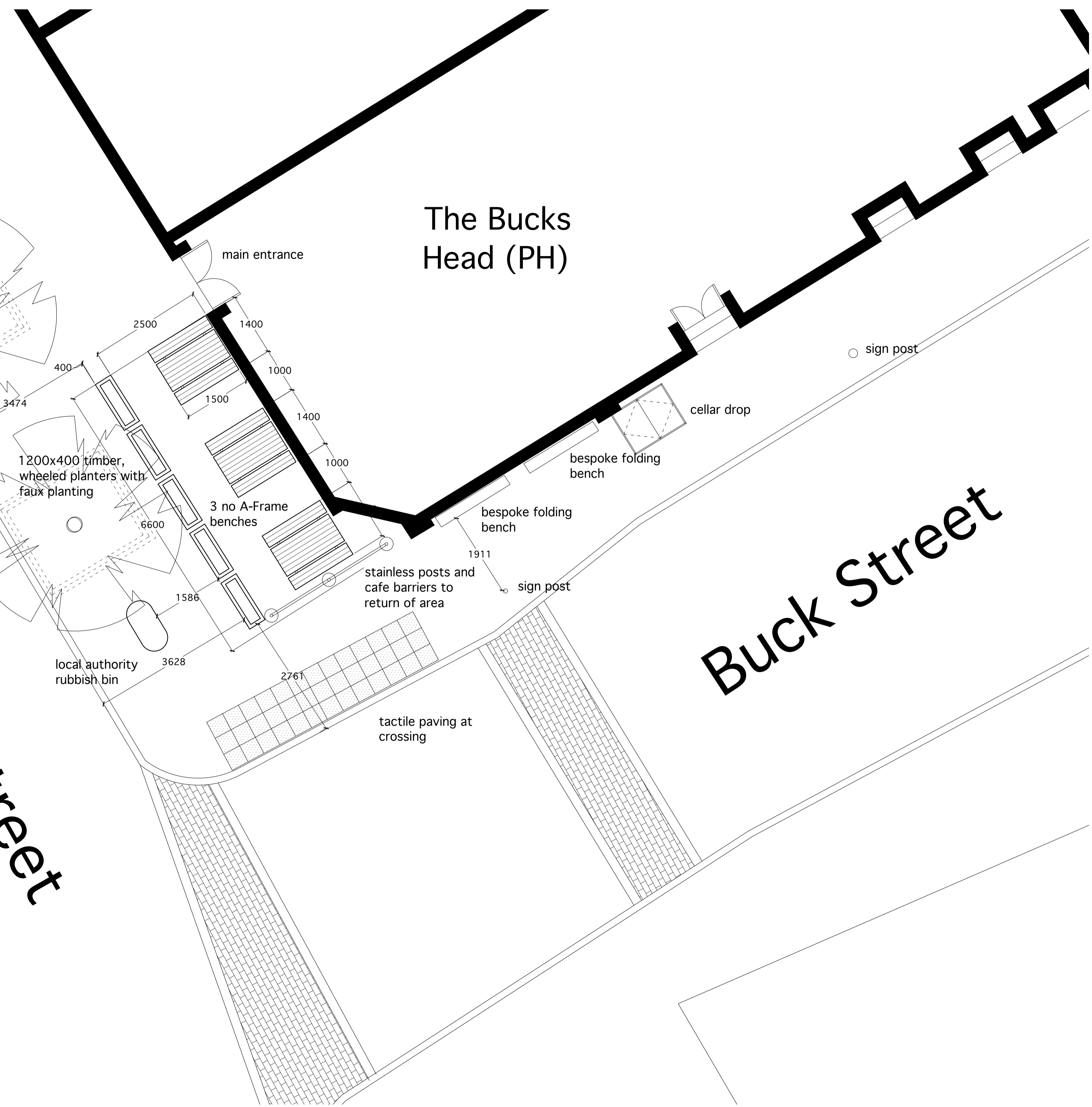
proposed side barriers - stainless steel posts with branded cafe barrier inserts - 1400mm long x 1000mm high
