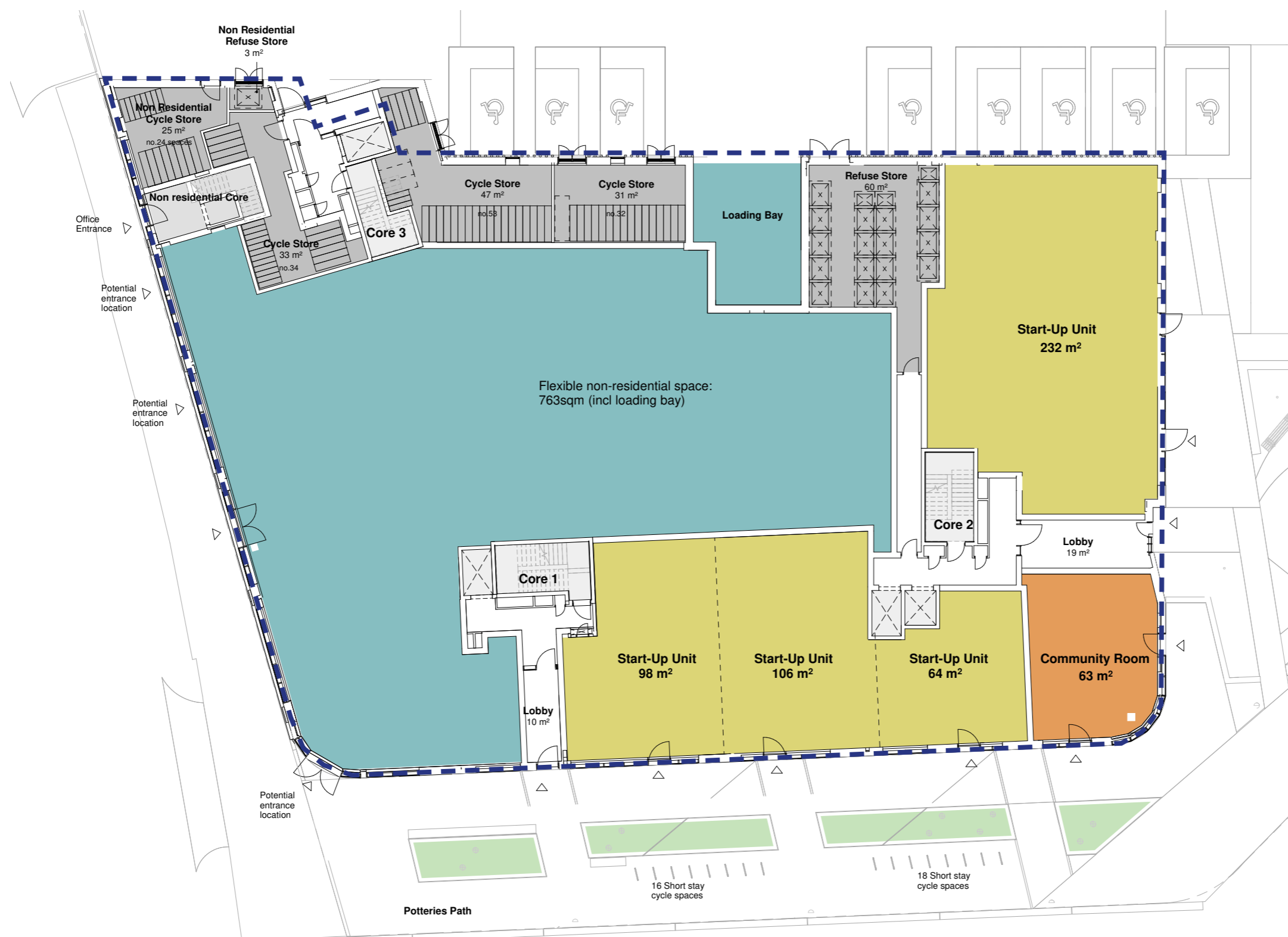
Proposed Ground Floor Plan - Scale 1:250
