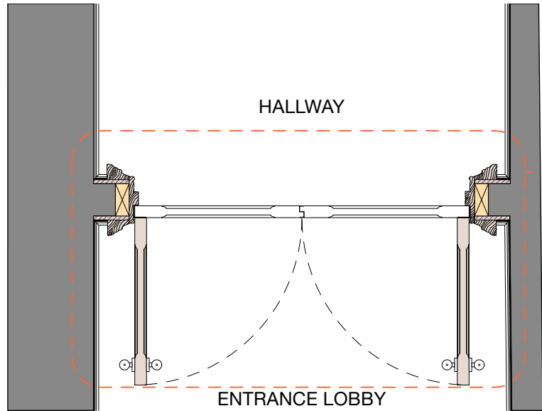
P Entrance Lobby Door Plan 1:20
