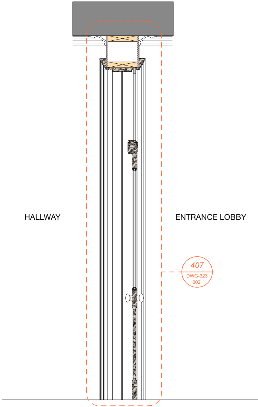
S Entrance Lobby Door Section 1:20
