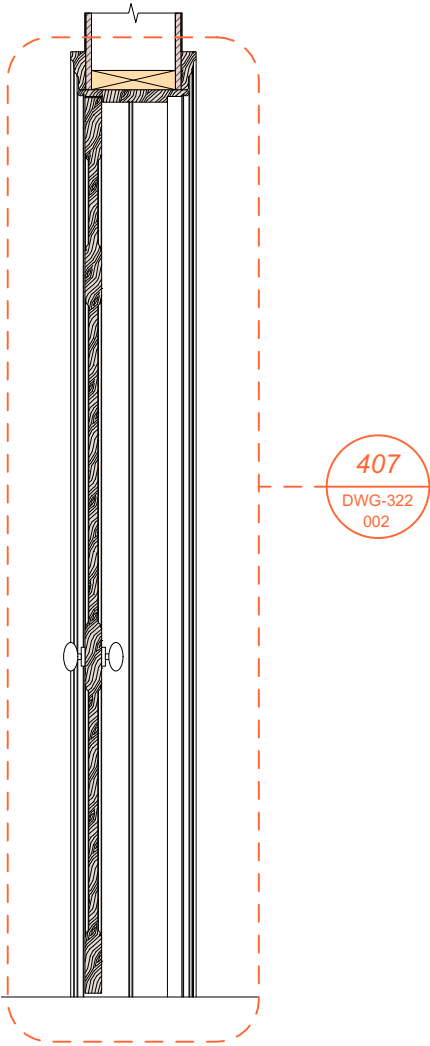
S First and Second Floor Door Section 1:20
