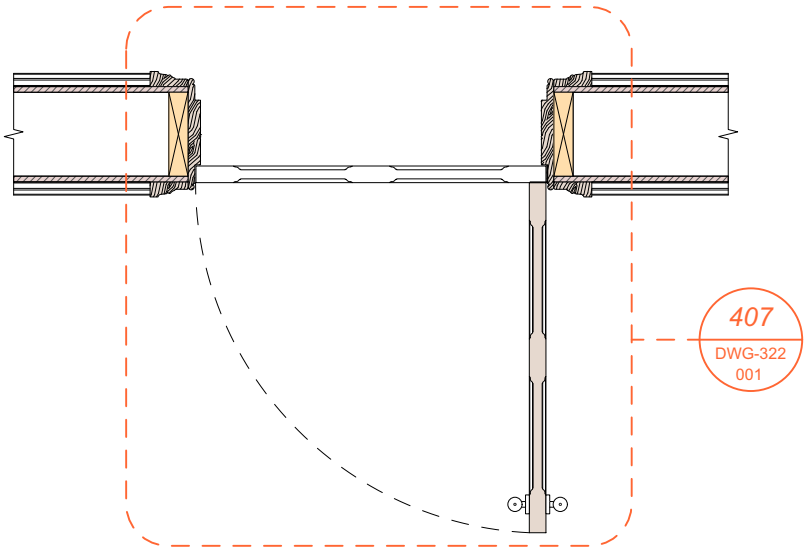
P First and Second Floor Door Plan 1:20
