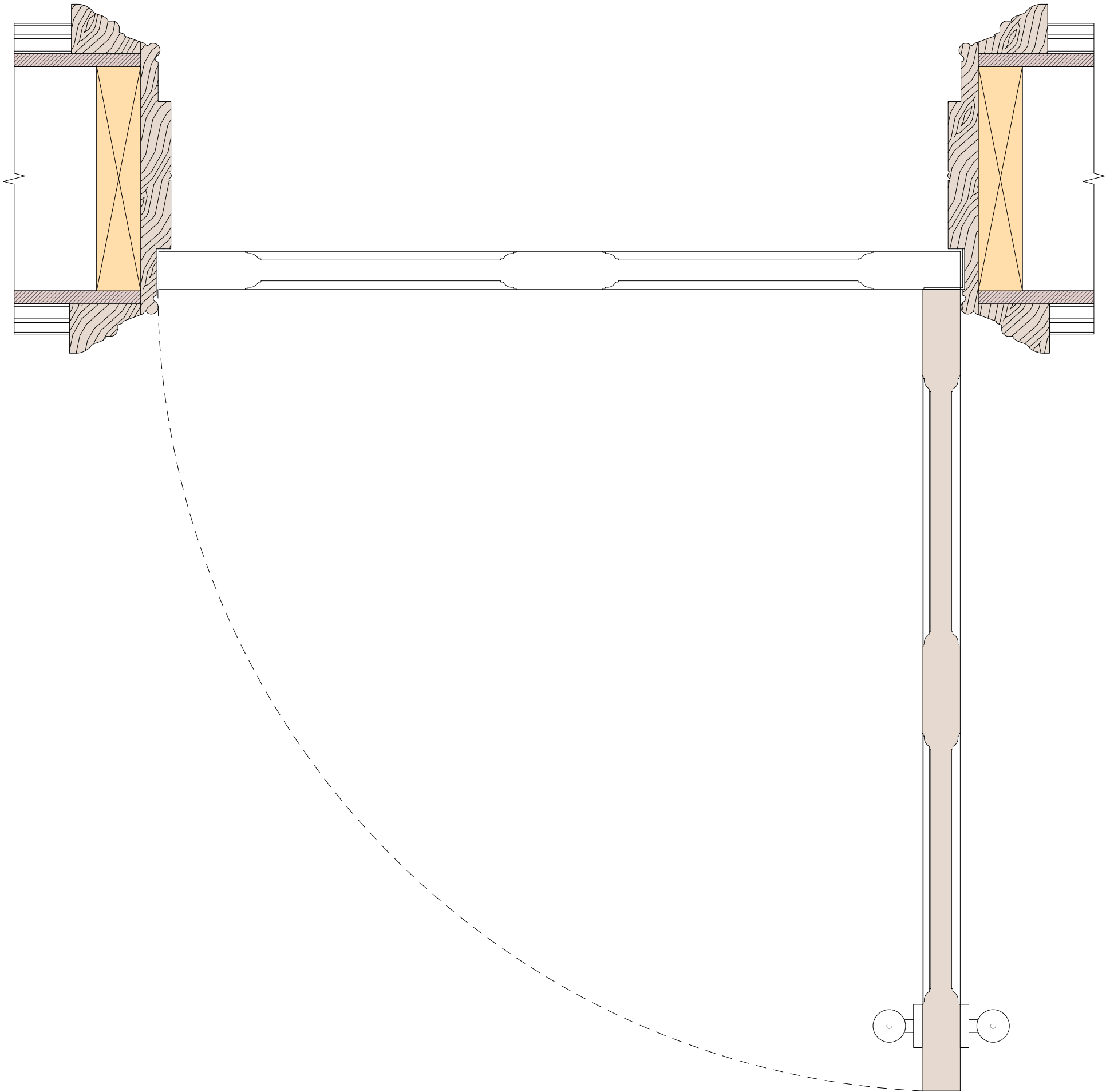
P Ground Floor Door Jamb Detail 1:5
