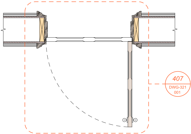
P Ground Floor Door Plan 1:20
