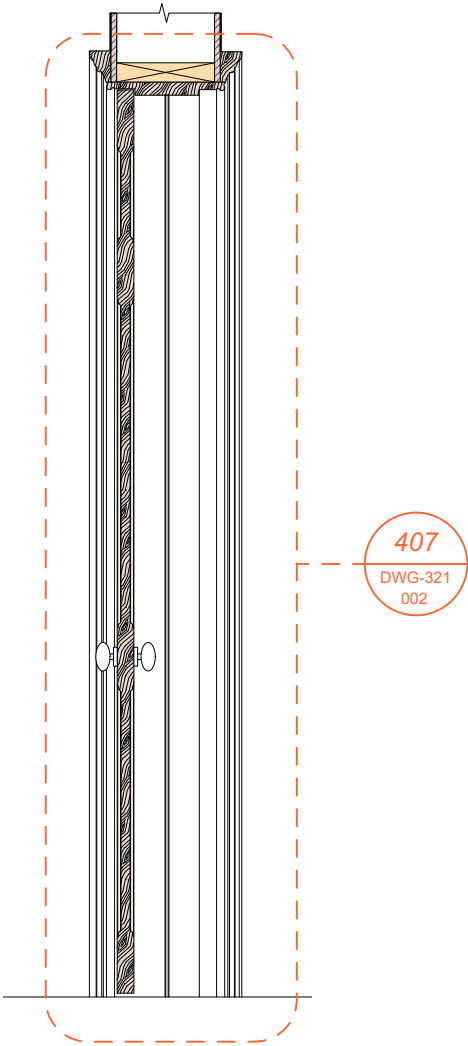
S Ground Floor Door Section 1:20
